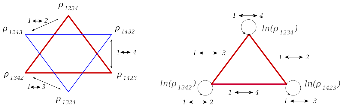
Figure 2. Symmetry properties of conformally invariant cross ratios. Each of the two triangles in the left-hand figure connects three cross ratios. The cross ratios associated with the two triangles are related by inversion, and one moves between the two triangles with odd permutations of momentum labels. The right-hand figure shows the resulting antisymmetry of the logarithms of the three conformally invariant cross ratios under permutations. The three variables L_{1234} , L_{1423} and L_{1342} transform into one another under permutations, up to an overall minus sign. For example, under the permutation 1 \leftrightarrow 2 , we have L_{1234} \rightarrow -L_{1423} , L_{1423} \rightarrow -L_{1234} , and L_{1342} \rightarrow -L_{1342} .
