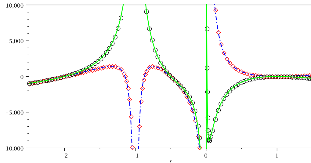
Figure 3. The logarithmic functions \Delta_4 with transcendentality \tau = 5 introduced in eqs. (5.30) and (5.31), respectively, in the case of a four-parton amplitude with no recoil. In each case we separately display the real (dot-dash) and imaginary (solid line) parts as a function of the ratio r , defined in eq. (A.1), multiplying the color coefficient f^{ade} f^{cbe} after the Jacobi identity has been taken into account, as in eq. (A.3). In each case symbols represent eq. (5.30) while the lines stand for eq. (5.31). The plot demonstrates that the two are identical once the Jacobi identity is taken into account.
