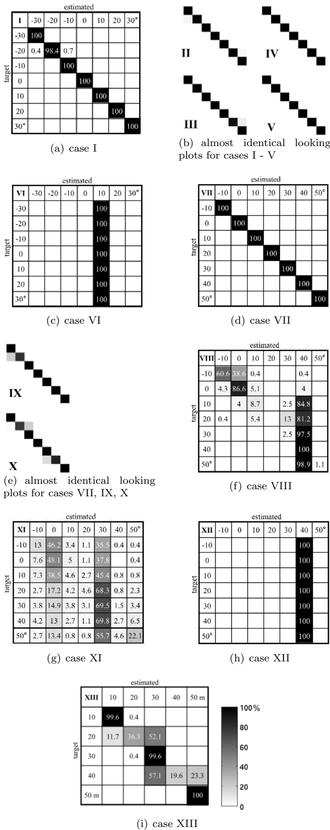
Fig. 3: DNN performance of the testing. The average of 100 ms (10 frames) is rated as one decision of the network.
