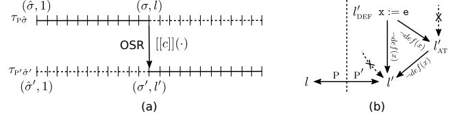
Figure 4. (a) OSR mapping allowing a transition from program \mathbb{P} at l to program \mathbb{P}' at l' . (b) Algorithm reconstruct identifies an assignment x := e at l'_{\text{DEF}} that reaches both l' and l'_{\text{AT}} , and no other definition of x is possible.
