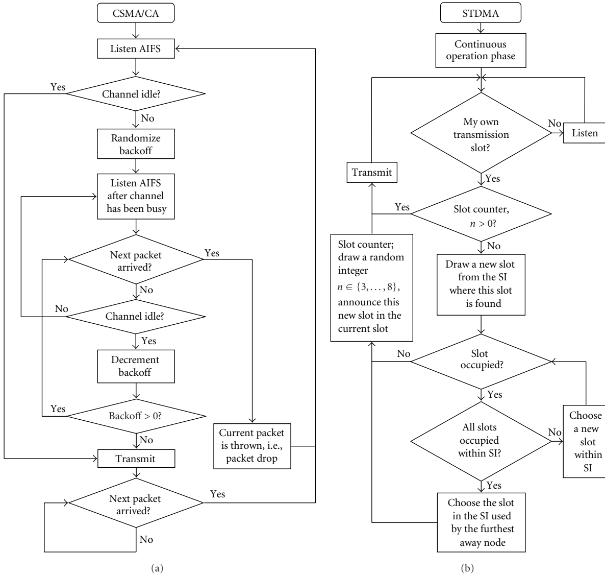
FIGURE 2: The two MAC procedures examined in this paper using a data traffic model with broadcasted time-driven messages at predetermined heartbeat rates, (a) the CSMA procedure according to 802.11p and (b) continuous operation phase of STDMA.
