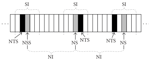
FIGURE 3: The frame structure for one node. The NSS and NSs are equally spaced with an interval of size NI. The SI parameter is also fixed.
