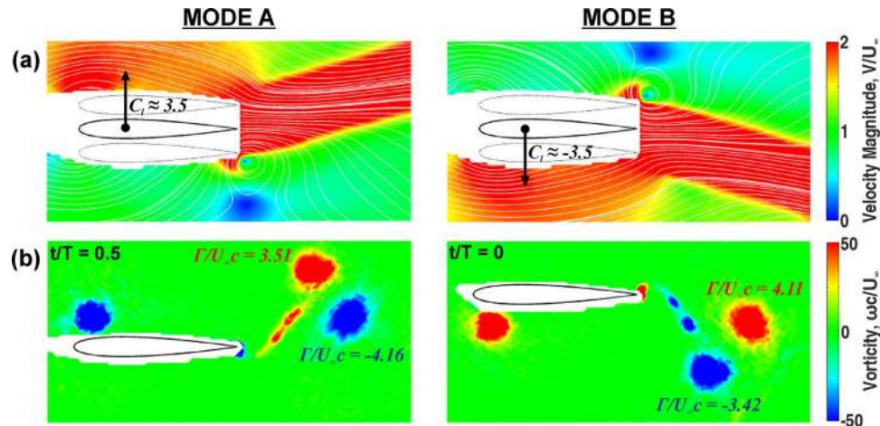
FIG. 1. (a) Time-averaged velocity showing deflected jets for a NACA0012 airfoil at \alpha = 0^\circ and \text{Re} = 10000 . The direction of the deflected jet determines the positive or negative lift coefficient and is characterised by asymmetry in the trailing-edge vortex strength; (b) phase-averaged vorticity (adapted from Cleaver et al. 8 ). Reprinted with permission from Cleaver et al. , J. Fluid Mech. 708 , 349–376 (2012). Copyright 2012 Cambridge University Press.
