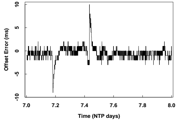
Figure 11. Radio Clock Offset Errors
