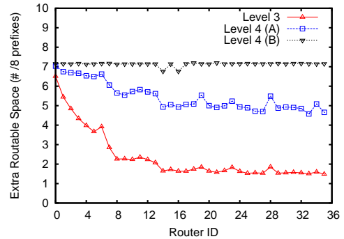
Fig. 8. Extra Routable Address Space (RouteViews Tables)
