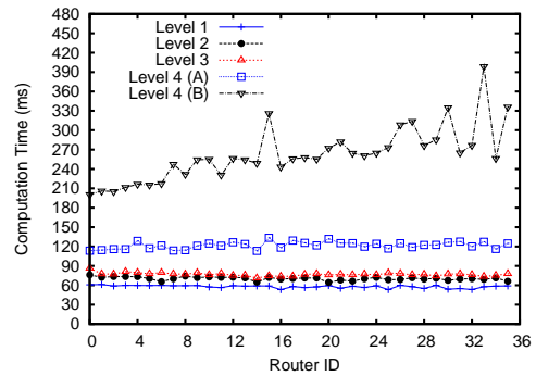
Fig. 7. Computing Time (RouteViews Tables)
