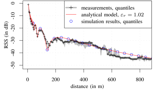
Figure 4. Measurement results of received signal strength vs. distance between sender and receiver (median, 1%, and 99% quantiles), overlaid with the calibrated Two-Ray Interference model and simulation results.
