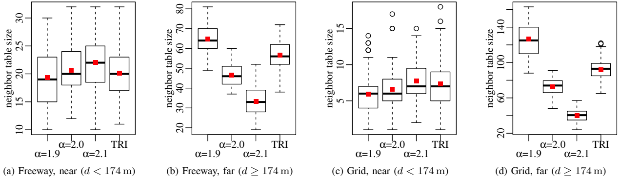
Figure 6. Distribution of nodes' neighbor table sizes (considering either only near or far neighbors). Results from the 1D Freeway and 2D Grid scenarios (1 Hz beacon interval), plotted for three empirical adaptations of the Free-space path loss model, as well as for the Two-Ray Interference model.
