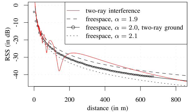
Figure 5. Model comparison for the Free-space model using different \alpha values and the Two-Ray Interference model. For d_c < 866.6 \text{ m} , results for \alpha = 2.0 and for the simplified Two-Ray Ground model are identical.
