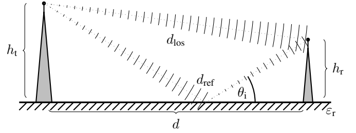
Figure 1. Conceptual model of ground reflection causing distance-dependent constructive and destructive signal interference effects at the receiver.
