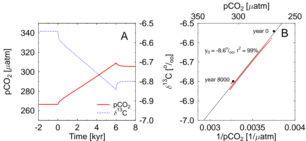
Fig. 7. Effects of a linear decrease in terrestrial carbon storage by 500 PgC (left: p\text{CO}_2 , \delta^{13}\text{C} ; right: Keeling plot). Regressions in the Keeling plots are performed over the whole time period.
