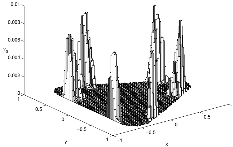
FIG. 6.6. Approximation of the invariant measure for \alpha = -1.7 .
