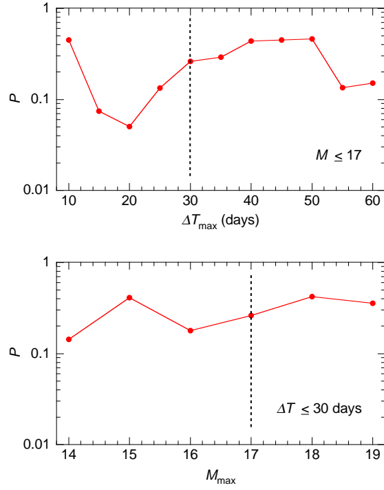
Fig. 1.— Gamma-ray burst/ supernova correlation significance P (small number indicates higher significance) as a function of the supernova magnitude selection M \leq M_{\max} and temporal window 0 \leq \Delta T \leq \Delta T_{\max} . Dashed lines indicate the baseline search criteria.
