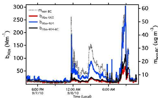
Fig. 3. Time series of measured 404 nm and 658 nm absorption of ambient particles (blue and red lines), 404 nm thermo-denuded absorption (black) and non-refractory aerosol mass (dashed grey line).
