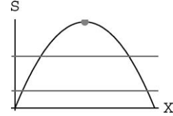
Figure 2. Strong causality.
