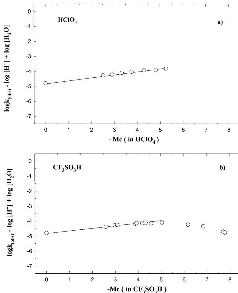
Figure 2 Beckmann rearrangement of 2,4,6-trimethylacetophenone oxime in \text{HClO}_4 (range 52–72 wt%) and in \text{CF}_3\text{SO}_3\text{H} (range 69–100 wt%) at 25^\circ\text{C} : a) Plot of \{\log k_{\text{obs}} - \log[\text{H}^+] + \log[\text{H}_2\text{O}]\} vs \text{Mc} in \text{HClO}_4 ; intercept = -4.8 , slope = 0.2 . b) Plot of \{\log k_{\text{obs}} - \log[\text{H}^+] + \log[\text{H}_2\text{O}]\} vs \text{Mc} in \text{CF}_3\text{SO}_3\text{H} ; (intercept = -4.8 , slope = 0.18 in the range 50–90 wt%). Values of \log k_{\text{obs}} for the formation of intermediate in \text{HClO}_4 from Ref. [7]; in \text{CF}_3\text{SO}_3\text{H} from present work. Values of \text{Mc} and \log[\text{H}^+] in \text{HClO}_4 and in \text{CF}_3\text{SO}_3\text{H} from Ref. [11].
