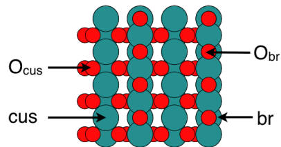
FIG. 1: Top view of the (110) rutile surface together with the different considered adsorption sites and the unit cell. Here, cus denotes the coordinately unsaturated site on top of a fivefold coordinated metal atom, the br denotes the bridge site between two fourfold coordinated metal atoms [note this corresponds to a (110) surface without O atoms], \text{O}_{\text{br}} denotes the site on top of an O in the bridge site, \text{O}_{\text{cus}} denotes the site on top of an O in the bridge site between two fivefold metal atoms.
