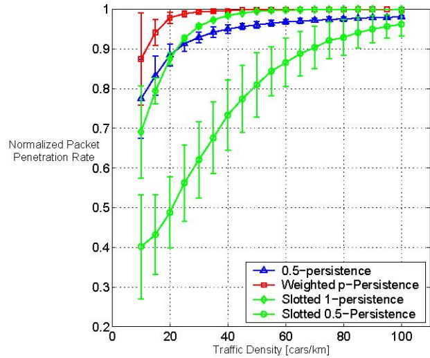
(b) Normalized Packet Penetration Rate
