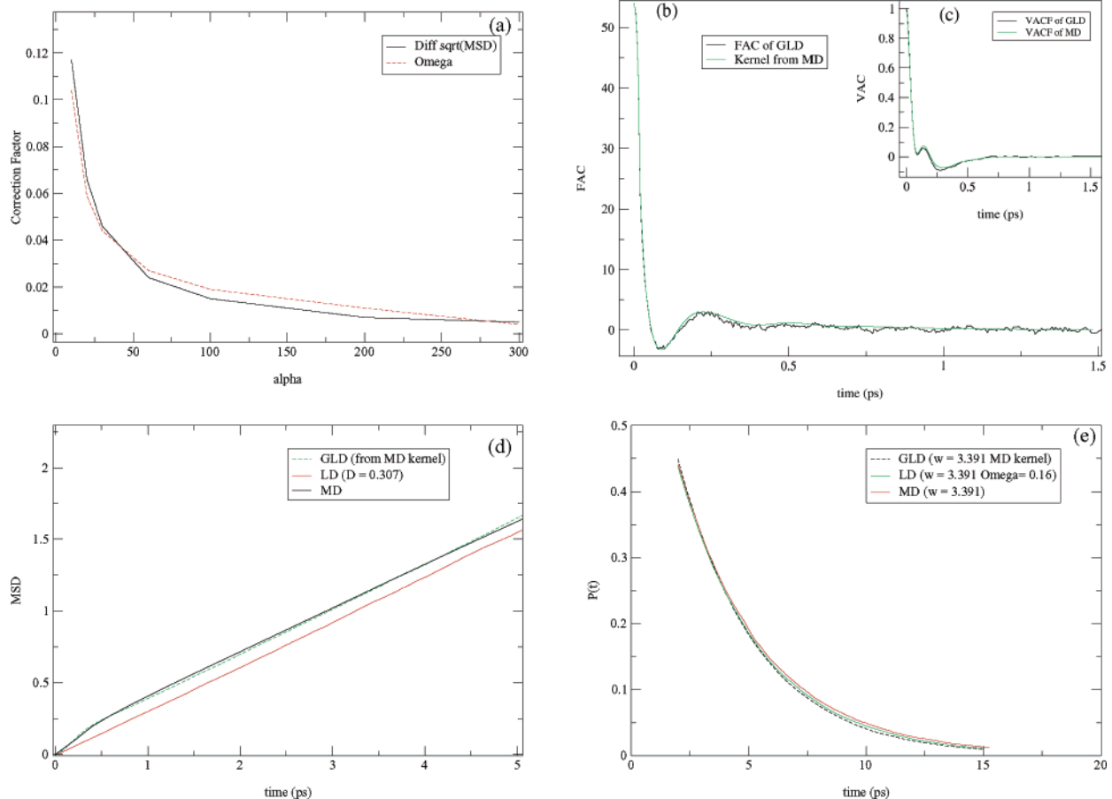
Figure 2. (a) Plot of memory correction factor vs inverse of characteristic time. The dash line and solid line are the correction factors \omega from the GLD and LD and the biggest difference of \sqrt{\langle \Delta z(t)^2 \rangle} , respectively. The static friction corresponds to D = 0.25 \text{ \AA}^2/\text{ps} , T = 300 \text{ K} , and water molecule mass. (b) Friction kernel. The solid line is calculated from the velocity autocorrelation function of MD by solving the Volterra equation numerically, see cited reference 21 for details. From the second fluctuation–dissipation theorem, the relationship between the friction kernel and the random force autocorrelation function (FAC) can be established as \zeta_{zz}(t) = \beta \langle R(0)R(t) \rangle , where \beta = 1/(kT) and R_z is the random force. The curve of FAC is scaled by \beta . (c) Velocity autocorrelation function (VAC) from the molecular simulation and the GLD. (d) Mean-square displacement. The GLD simulation with the real friction kernel can almost reproduce the same MSD curve as the real MD simulation. The difference of the \sqrt{\langle \Delta z(t)^2 \rangle} is obvious. (e) Survival probability from MD, GLD with real friction kernel, and Langevin dynamics with width corrected using mean square displacement prescription. The coincidence of these curves proves the accuracy of the numerical kernel and the memory correction.
