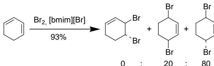
Scheme 18. Bromination of 1,3-cyclohexadiene in [bmim][Br] at room temperature.
