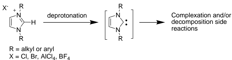
Scheme 3. The non-innocent nature of imidazolium-based ILs.
