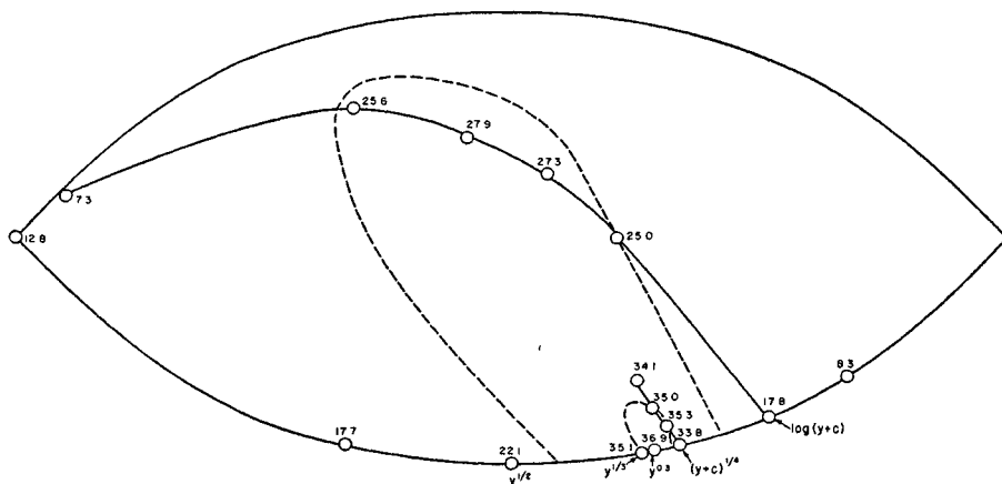
FIG. 4. Use of Fig. 3 to illustrate approximate normality of simple transforms of \chi^2_6 . (Large entries indicate good approximations. Scaled by y_0 = 0.6 , e_0 = 0.5 .)
