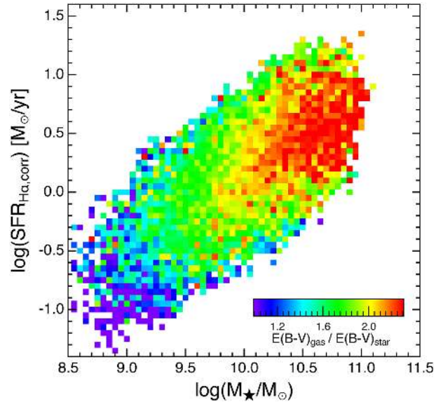
Fig. 12. Same plot as figure 10, but here we use H\alpha -based SFRs instead of UV+IR SFRs . In this plot it can be seen that the E(B - V)_{\text{gas}}/E(B - V)_{\text{star}} ratio is higher at the massive end, with \log(M_*/M_\odot) \gtrsim 10.5 , while the visual impression on the trend across the SF main sequence is slightly different from that of figure 10, particularly at the low-mass/low- SFR end (see text for more details). (Color online)
