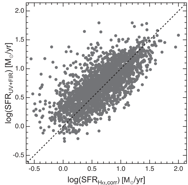
Fig. 2. SFRs derived from UV and FIR photometry ( SFR_{\text{UV+FIR}} ) of our new AKARI–SDSS–GALEX sample plotted against their H\alpha -based SFRs with corrections for fiber/aperture effects as well as the dust attenuation effect ( SFR_{H\alpha, \text{corr}} ; see text for details). As shown by Koyama et al. (2015) with the older version of the catalog, this plot demonstrates good agreement between the two independently measured SFRs .
