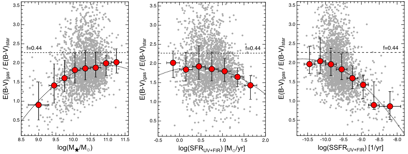
Fig. 6. Extra attenuation toward nebular emission quantified by the E(B - V)_{\text{gas}}/E(B - V)_{\text{star}} ratio, plotted against stellar mass (left), SFR (middle), and specific SFR (right) for our AKARI-SDSS-GALEX sample. The gray circles indicate individual AKARI-SDSS-GALEX galaxies, and the red circles with error bars show their median data points computed for a constant 0.3 dex bin, with the y -axis error bars representing their 25%–75% distribution. We note that a wider bin size is adopted at the lowest-mass and highest- sSFR bins so that each bin has a sufficient ( >15 ) number of galaxies. The error bars on the x -axis indicate the adopted bin size. The dotted-line curve drawn in each panel shows the best-fit polynomial function computed for the median data points weighted by \sigma/\sqrt{N} for each bin, and the horizontal dashed line indicates the canonical value of E(B - V)_{\text{star}}/E(B - V)_{\text{gas}} = 0.44 for reference. (Color online)
