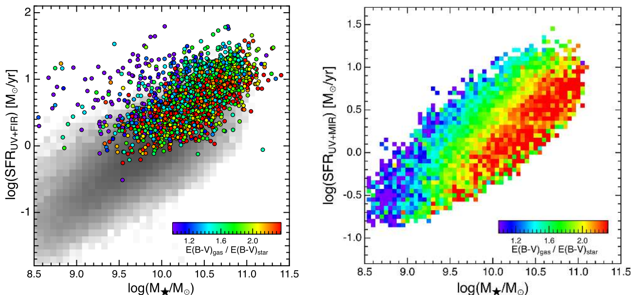
Fig. 10. Extra attenuation toward nebular regions across the SFR-M_* diagram for the AKARI-SDSS-GALEX sample (left) and for the WISE-SDSS-GALEX sample (right). In the left panel we show the individual data points of the AKARI-SDSS-GALEX sample with color coding indicating the E(B - V)_{\text{gas}}/E(B - V)_{\text{star}} ratio, and the gray-scale density plot shows the distribution of the parent SDSS-GALEX sample (same as figure 3). For the right panel we compute the average E(B - V)_{\text{gas}}/E(B - V)_{\text{star}} ratio of the WISE-SDSS-GALEX sample at each position on this diagram by dividing each panel into 60 \times 60 sub-grids. We note that we require here a minimum sample size of N_{\text{galaxy}} = 4 for each pixel, and thus the data points seen at the top-left corner of the left panel (i.e., low-mass galaxies with high SFR ) are not seen in the right panel. The two plots are broadly consistent with each other in the sense that the E(B - V)_{\text{gas}}/E(B - V)_{\text{star}} ratio becomes largest at the low- SFR side. (Color online)
