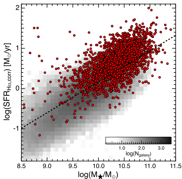
Fig. 3. AKARI(FSCv1)–SDSS–GALEX galaxy sample plotted on an SFR – M_* diagram (red circles). The gray-scale density plot indicates the distribution of the whole SDSS–GALEX matched SF galaxy sample. To create this plot we divide the panel into 40 \times 40 sub-grids, and compute the number counts of galaxies in each pixel. We note that M_* and SFR_{H\alpha, \text{corr}} are derived in the same way for both AKARI-detected and undetected sources. (Color online)
