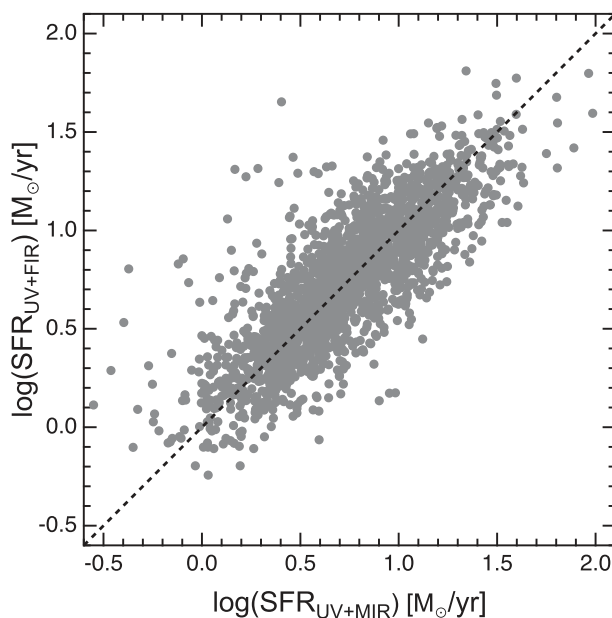
Fig. 7. SFRs derived from AKARI FIR photometry (subsection 2.2) plotted against SFRs from WISE 22 \mu\text{m} data taken from the public GSWLC catalog by Salim et al. (2016) for galaxies identified in both our AKARI-SDSS-GALEX sample and the GSWLC catalog, taking into account the different IMF assumptions. The two SFR measurements show good agreement with each other.
