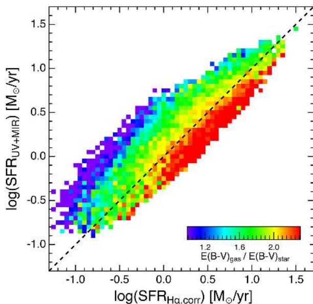
Fig. 13. Average extra reddening toward nebular regions, E(B - V)_{\text{gas}}/E(B - V)_{\text{star}} , at each position on the SFR_{\text{H}\alpha} – SFR_{\text{UV+MIR}} diagram. There is a clear trend that galaxies showing SFR_{\text{H}\alpha} > SFR_{\text{UV+MIR}} tend to have higher levels of E(B - V)_{\text{gas}}/E(B - V)_{\text{star}} . (Color online)
