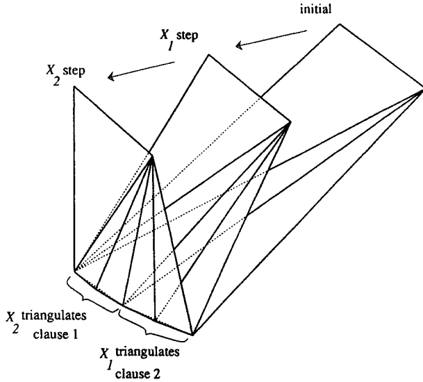
Fig. 15. The interface sweeping across the polyhedron. After each step, everything to the right of the interface has been triangulated.
