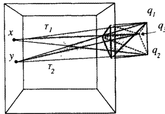
Fig. 10. Tetrahedra T_1 and T_2 overlap; at most one of them can appear in any triangulation.
