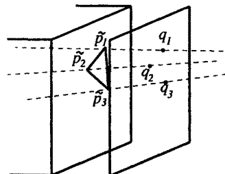
Fig. 7. Placing q_1, q_2, q_3 .
