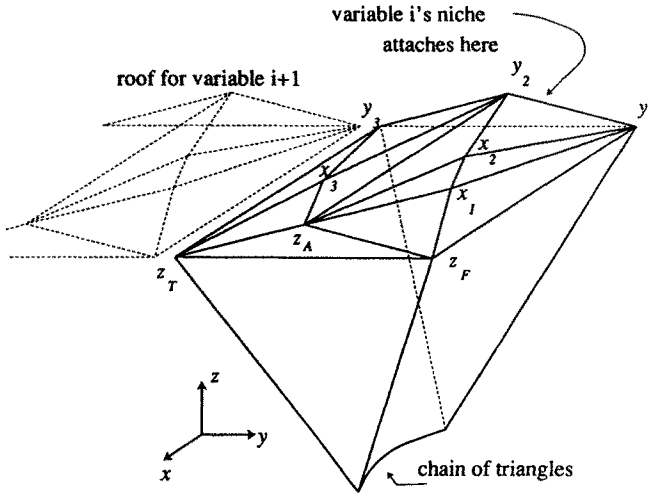
Fig. 16. A variable's roof (seen from the "right").
