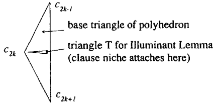
Fig. 29. Clause niches are attached to base triangles.
