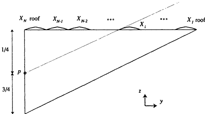
Fig. 30. Front view of polyhedron, showing plane (dotted) bounding variable X_i 's roof (not to scale).
