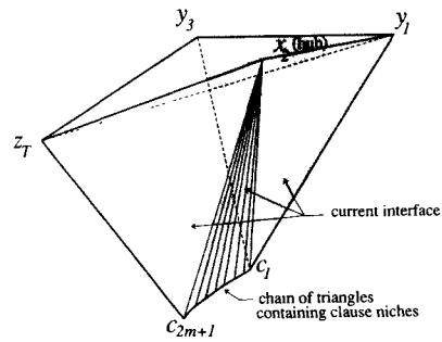
Fig. 20. Shaded triangles to form tetrahedra with z_T .
