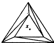
Fig. 3. Entire prism visible from the center x_0 of the top face.
