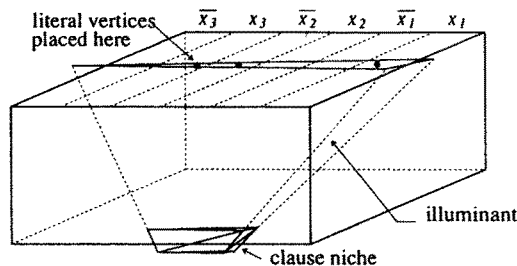
Fig. 12. Regions of polyhedron corresponding to variables, niche for clause (\bar{X}_1 + \bar{X}_2 + X_3) , and placement of three corresponding literal vertices.
