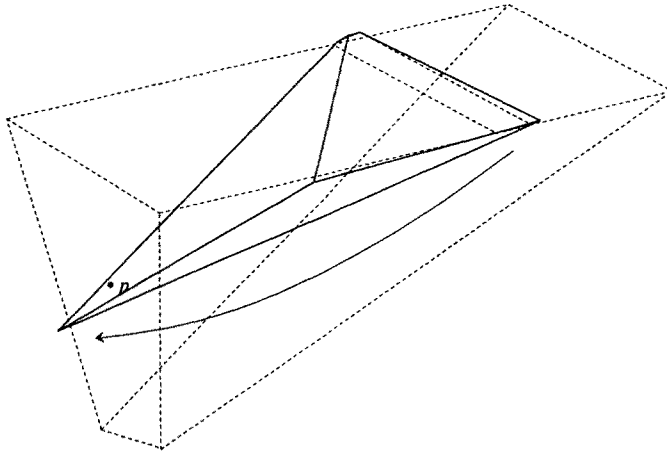
Fig. 36. Illuminants of variable niches “stretch” so as to include the point p .
