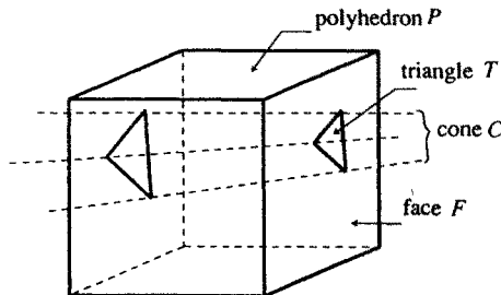
Fig. 6. The setting for the Illuminant Lemma.
