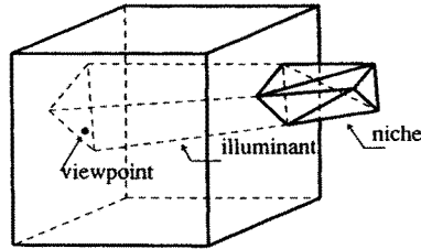
Fig. 5. A niche attached to a cube.
