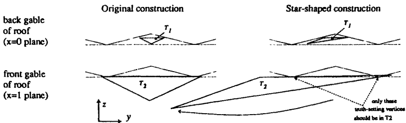
Fig. 37. More details of variable niche stretching (the roof gables are shown dotted).
