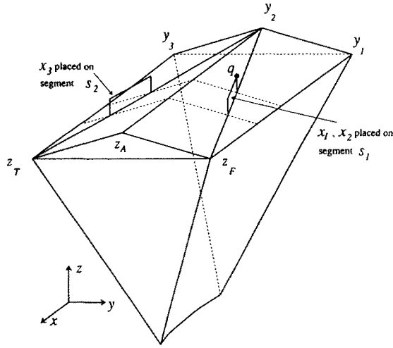
Fig. 31. Placement of x_1, x_2, x_3 (for i th variable, i superscripts omitted).
