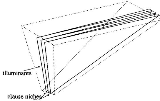
Fig. 28. The shape of the clause niche illuminants. The clause niches themselves are very small, along the bottom.
