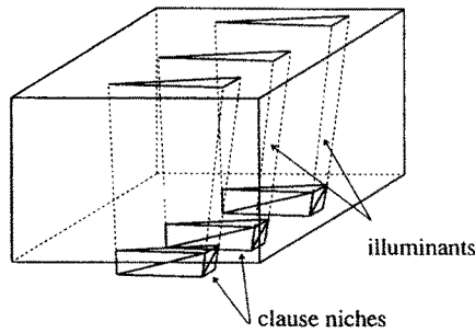
Fig. 11. Clause niches attached to polyhedron P .
