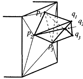
Fig. 9. The constructed niche.
