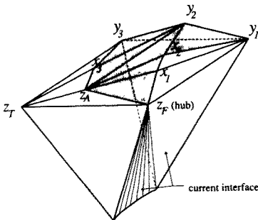
Fig. 17. Shaded triangles to form tetrahedra with z_T .
