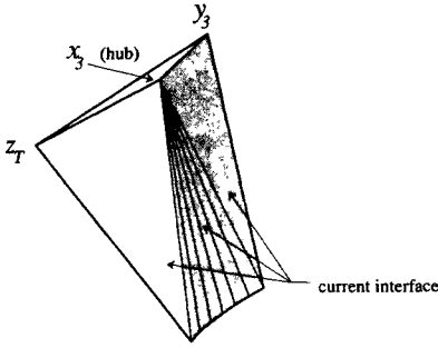
Fig. 24. Shaded triangles to form tetrahedra with z_T .
