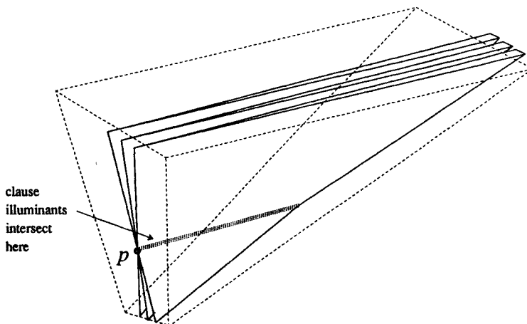
Fig. 35. To produce a star-shaped polyhedron: illuminants of clause niches “tilt” slightly so as to intersect (triple dashed lines).
