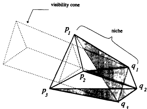
Fig. 4. Visibility cone for a niche.
