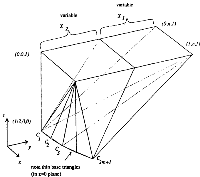
Fig. 14. Starting point for the polyhedron construction.
