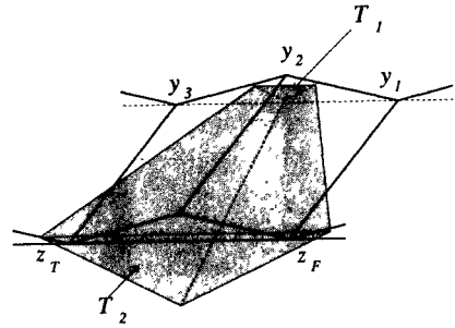
Fig. 25. The cone C defined by the two similar triangles T_1 and T_2 .
