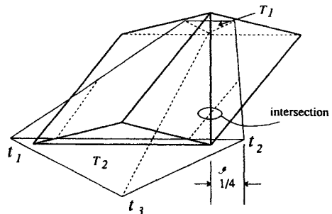
Fig. 27. Specification of T_2 . The cone C intersects segment y_2z_F exactly three-quarters of the way from y_2 to z_F .
