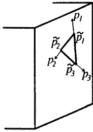
Fig. 8. Placing p_1, p_2, p_3 .
