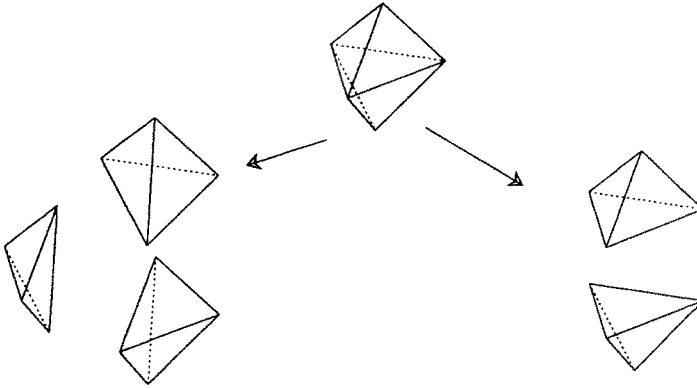
Fig. 1. The number of tetrahedra in a triangulation of a polyhedron is not unique.
