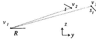
Fig. 33. The slope of v_1v_2 must be greater than the slope of v_1v_3 .
