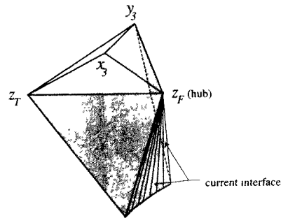
Fig. 23. Shaded triangles to form tetrahedra with x_3 .
