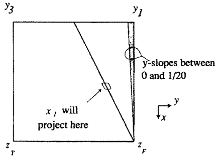
Fig. 34. In the z = 1 plane: shaded region shows where interface planes will intersect.
