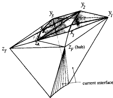
Fig. 22. Shaded triangles to form tetrahedra with z_F .
