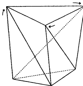
Fig. 2. A polyhedron that cannot be triangulated.
