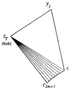
Fig. 21. Final interface after step for variable X .
