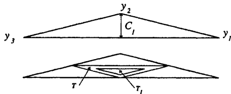
Fig. 26. In the x = 0 plane: the back gable of the roof (top), and the choice of T_1 within the back gable.
