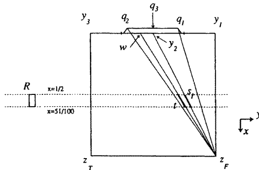
Fig. 32. Every line of sight from the segment s_1 to R must pass “beneath” the segment t .
