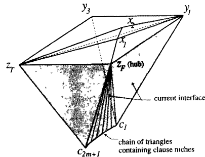
Fig. 18. Shaded triangles to form tetrahedra with x_1 .
