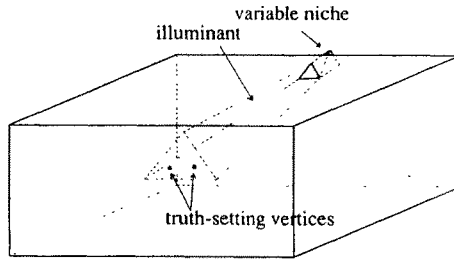
Fig. 13. Truth-setting vertices are viewpoints of variable niches.
