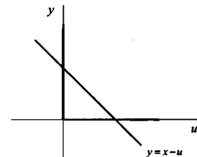
Fig. 4. A linear relation and complementarity conditions.
