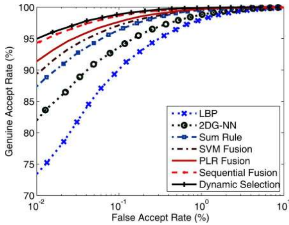
Fig. 6. ROC curves of the constituent face matchers, the proposed sequential fusion scheme, the dynamic selection algorithm, and some existing fusion algorithms.
