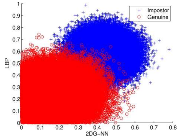
Fig. 7. Scatter plot shows that there is limited correlation between match scores obtained from LBP and 2DG-NN face recognition algorithms. Thus, score level fusion is expected to improve the matching performance.
