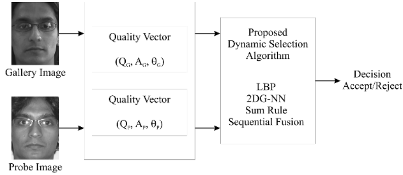
Fig. 4. Illustrating the steps involved in match score fusion of a multiclassifier face recognition system.
