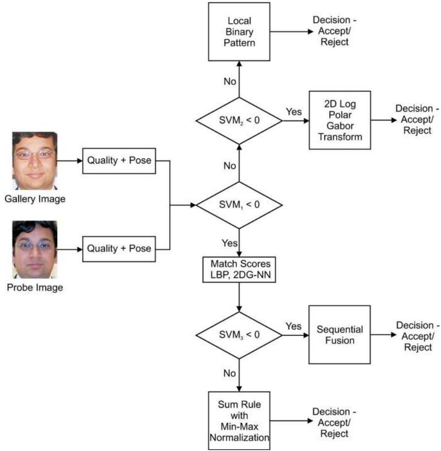
Fig. 2. Dynamic selection of biometric classifiers and fusion algorithms in the context of a face recognition application.
