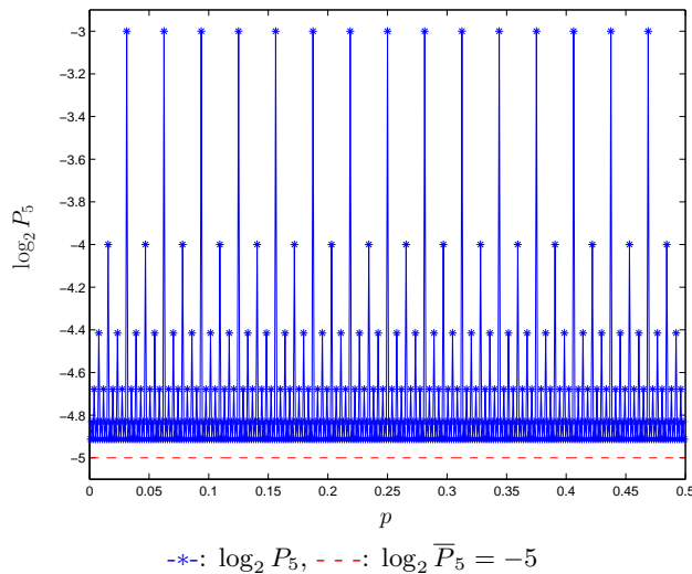
Fig. 5: \log_2 P_5 vs. p , where n = 10 and G_n(\cdot) = \text{floor}_n(\cdot) .
