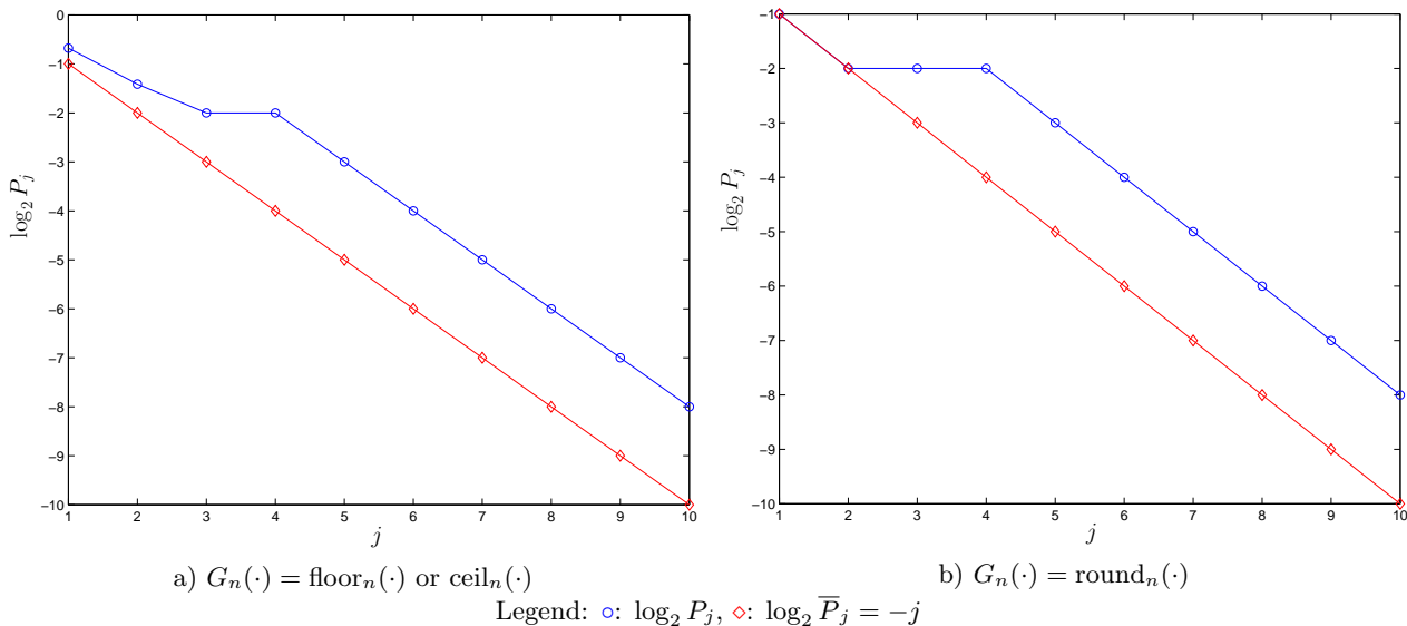
Fig. 3: The values of \log_2 P_j ( 1 \leq j \leq n ) when p = 3/16 \in V_4 and the finite precision n = 10 .
