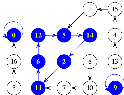
Fig. 2: The orbit-graph of the digital tent map F(x, p) with p = 3/2^4 in 4-bit finite precision (with round-off fixed-point arithmetic). The node marked with number i denotes the chaotic state of x = i/2^4 .
