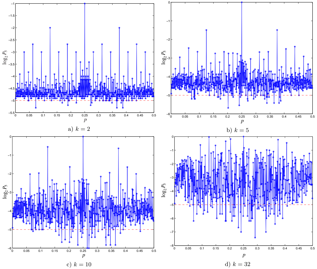
Fig. 6: \log_2 P_5 of \mathcal{F}_n^k(x) with respect to p , when k = 2, 5, 10, 32 (The dashed line denotes \log_2 \bar{P}_5 = -5 ).
