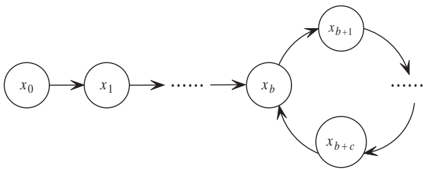
Fig. 1: A typical pseudo-orbit of a digital chaotic system.
