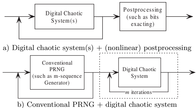
Fig. 9: Two common structures of chaotic PRNG.
