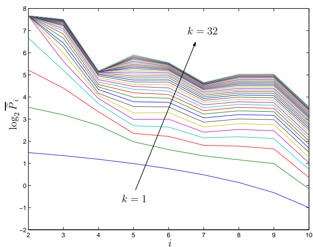
Fig. 7: \log_2 \bar{P}_i of \mathcal{F}_n^k(x) with respect to the resolution i , when k = 1 \sim 32 .
