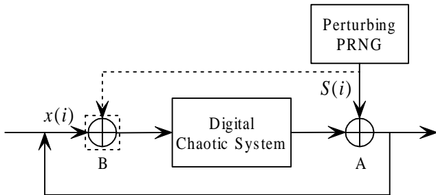
Fig. 8: Two available configurations of the perturbation-based algorithm.
