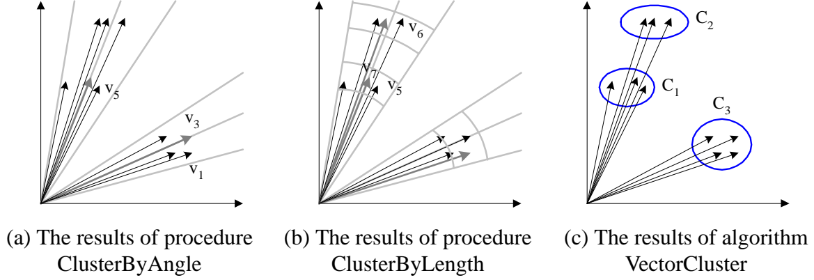
Figure 8: An example of motion vector clustering on \{M_1, M_2, \dots, M_{10}\}
