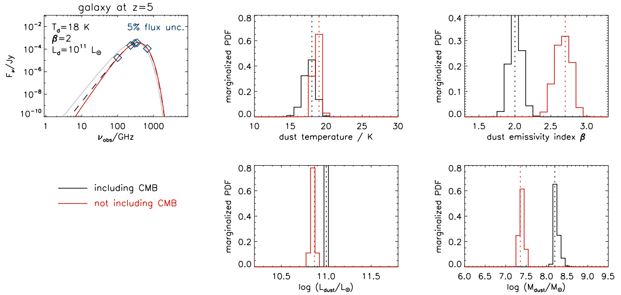
Figure 4. Comparison between fits to our fiducial model SED (intrinsic dust temperature of T_{\text{dust}}^{z=0} = 18 K, dust emissivity index \beta = 2 , total luminosity 10^{11} L_\odot , and total dust mass 1.6 \times 10^8 M_\odot ) at z = 5 , when including the effect of the CMB in the fit (in black) and when ignoring the effect of the CMB in the fit (in red). The “observed” fluxes are indicated as blue diamonds in the top-left panel; we use five common (sub-)millimeter bands at 100, 230, 300, 345, and 670 GHz. The gray SED is the intrinsic SED, i.e., before CMB corrections—the actual observed SED, i.e., with the effects of the CMB included as for Figure 2, is plotted as a dashed black line. The best-fit SED when fitting the blue fluxes but ignoring the effects of the CMB is plotted in red. The top right panels and the two bottom panels show the probability density functions (PDFs) of the constrained parameters (dust temperature, emissivity index, luminosity and mass) computed using a Bayesian fitting method (da Cunha et al. 2008), with the best-fit value for each parameter indicated by a vertical dashed line.
