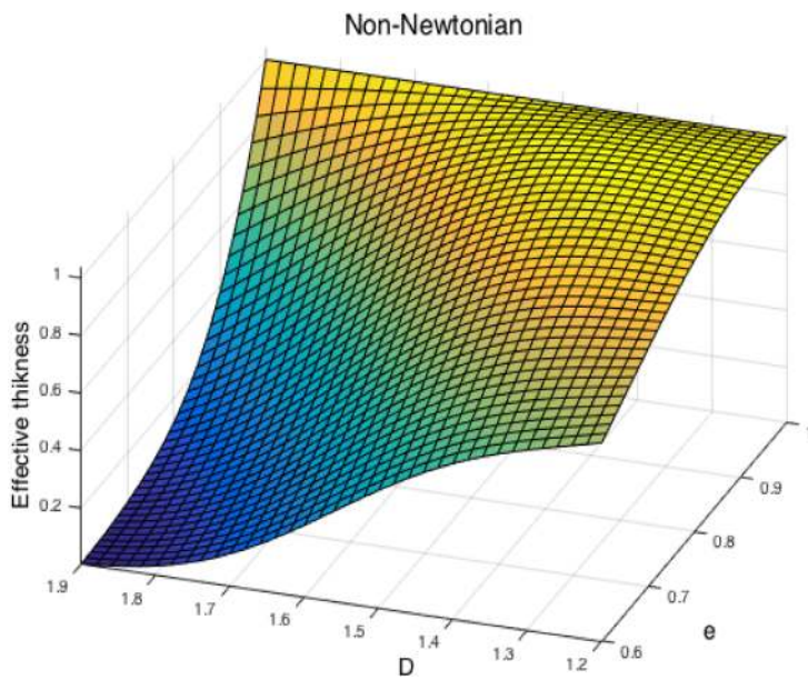
FIGURE 12 Effective thickness: non-Newtonian fluid [Colour figure can be viewed at wileyonlinelibrary.com ]
