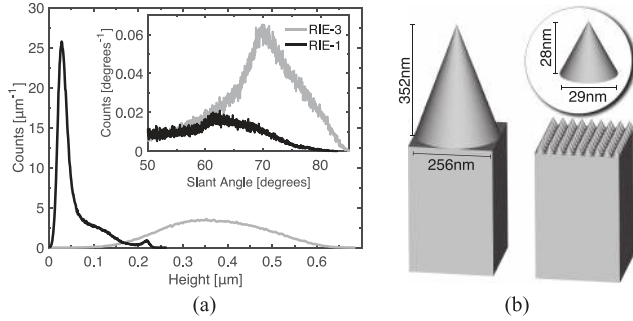
Fig. 8. (a) AFM height distributions for RIE-1(black) and RIE-3(gray). Inset: Corresponding slant angle distributions. (b) Schematics, of nanocones (presented on the same scale and on the same sized cuboid substrates) with dimensions calculated using the peak values from (a). Inset: zoom-in of the smaller nanocone.
