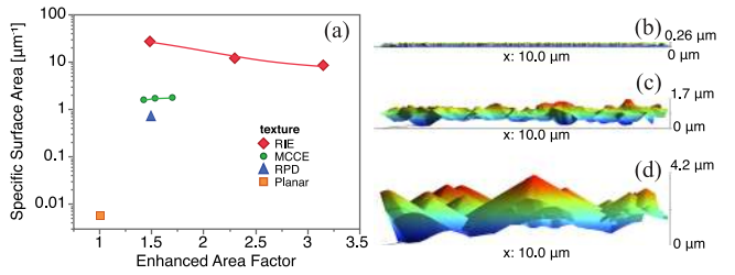
Fig. 6. (a) SSA versus EAF for various textured silicon samples and side-views of AFM scans presented on the same height scale for (b) B-Si RIE-1, (c) B-Si MCCE-2, and (d) RPD, which all have similar EAF values of \sim 1.5 .
