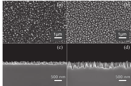
Fig. 4. Plan-view SEM images for RIE conditions with the (a) shortest etch time (RIE-1) and (b) the longest etch time (RIE-3) and their corresponding cross-sectional images, (c) and (d), shown directly below them.
