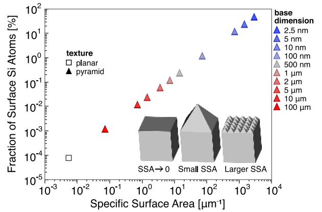
Fig. 1. Fraction of Si surface atoms versus SSA calculated for ideal pyramids ( \langle 100 \rangle base and \langle 111 \rangle faces), and for a reference planar surface. Pyramid base dimensions vary from 2.5 nm (largest SSA) to 100 \mu\text{m} (smallest SSA) while maintaining a fixed EAF ( \sim 1.7 ). Inset: schematics for planar and pyramid textures.
