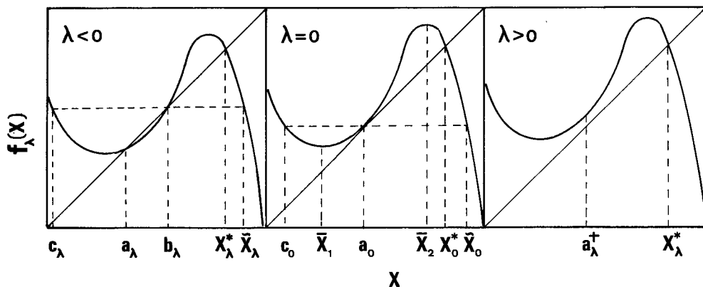
Fig. 1. — Graph of f_\lambda(x) .
