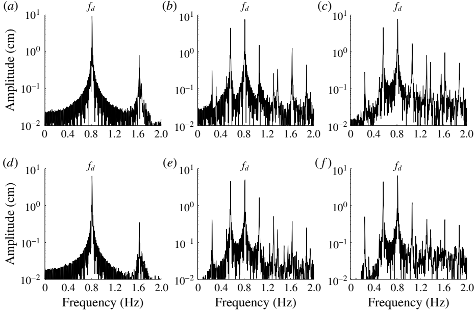
FIGURE 5. Fourier transforms of the experimental records in the time interval 50–300 s at the first gauge site ( a – c ), and the ninth gauge site ( d – f ), for case S1: ( a,d ) only third and fourth wave components generated; ( b,e ) the first four wave components generated; ( c,f ) all eight wave components generated. The dominant frequency is f_d = 0.81 Hz.
