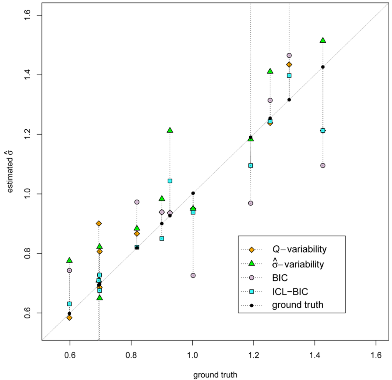
Figure 2. Estimates of \sigma obtained using the BIC-, ICL- and the \hat{\sigma} - and Q -variability-based methods plotted against the “ground truth”. For greater clarity of presentation, we have not plotted estimates obtained using the methods of Rajan et al. (2010) or Coupè et al. (2010).
