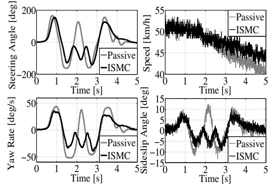
Figure 8. \delta(t) , r(t) and \beta(t) for the passive and active (in Normal mode) vehicles during an obstacle avoidance maneuver from an initial v = 51.5 km/h.
