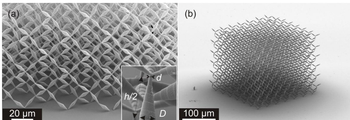
Fig.1: (a) Oblique-view electron micrograph of a polymer pentamode mechanical metamaterial fabricated by dip-in three-dimensional direct-laser-writing (DLW) optical lithography on a glass substrate with h = 16.15 \mu\text{m} and D = 3 \mu\text{m} . Importantly, the inset shows that the smallest accessible diameter of the connection regions of adjacent cones is about d = 0.55 \mu\text{m} . (b) Oblique-view electron micrograph of another polymer pentamode mechanical metamaterial with 7 \times 7 \times 6 face-centered-cubic unit cells (hence total size 261 \mu\text{m} \times 261 \mu\text{m} \times 224 \mu\text{m} ) and with h = 16.15 \mu\text{m} , D = 3 \mu\text{m} , and d = 1 \mu\text{m} . After Ref. [15].
