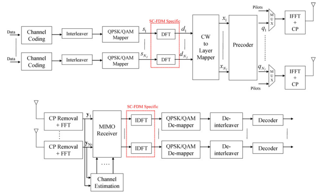
Fig. 1. Simplified OFDM/SC-FDM block diagram
