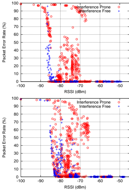
Fig. 2. Error rate vs. RSSI (1, 11 Mbps resply.)
