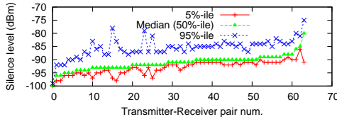
Fig. 4. Noise levels in Roofnet data (1 Mbps)
