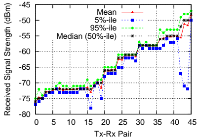
Fig. 8. Variation in the RSSI
