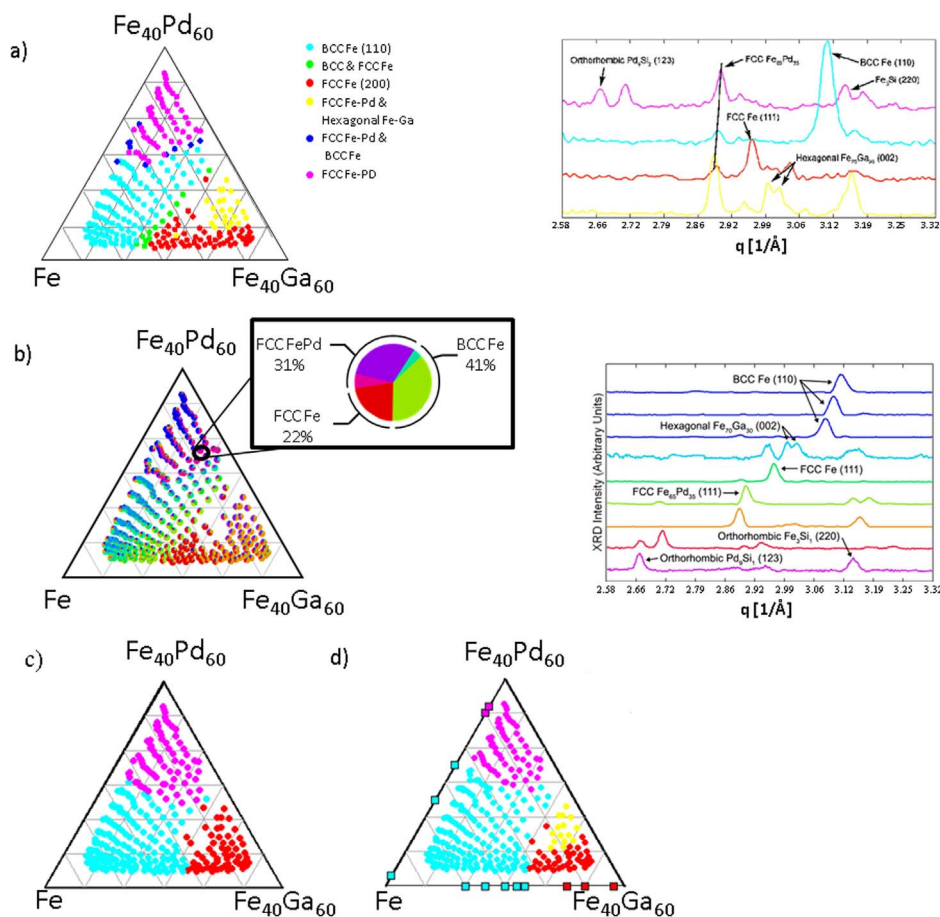
Figure 2 | Comparison of clustering results using different machine learning techniques applied to diffraction data taken from a Fe-Ga-Pd composition spread in the Fe-rich region. (a) Hierarchical cluster analysis clustering of diffraction pattern data (left); representative diffraction patterns from major cluster groups are plotted on the right; Reproduced from Ref. [30]. (b) Non-negative matrix factorization (NMF) analysis provides the positive principle components of the diffraction patterns. NMF gives deconvolution of patterns into components corresponding to peaks from pure phases, and accordingly, pie-charts are obtained at each average composition spot (left); peaks from basis patterns are then identified (right); Reproduced from Ref [31]. (c) High-speed mean shift theory based structural phase distribution analysis of experimental data using a suboptimal choice of bandwidth parameters. (d) High-speed MST results for experimental diffraction pattern data (ternary data points) and simulated data based on ICSD entries (square points along the binary lines) using the same suboptimal choice of bandwidths as in (c). ICSD based simulated data provides improved cluster stability despite suboptimal bandwidth choice.
