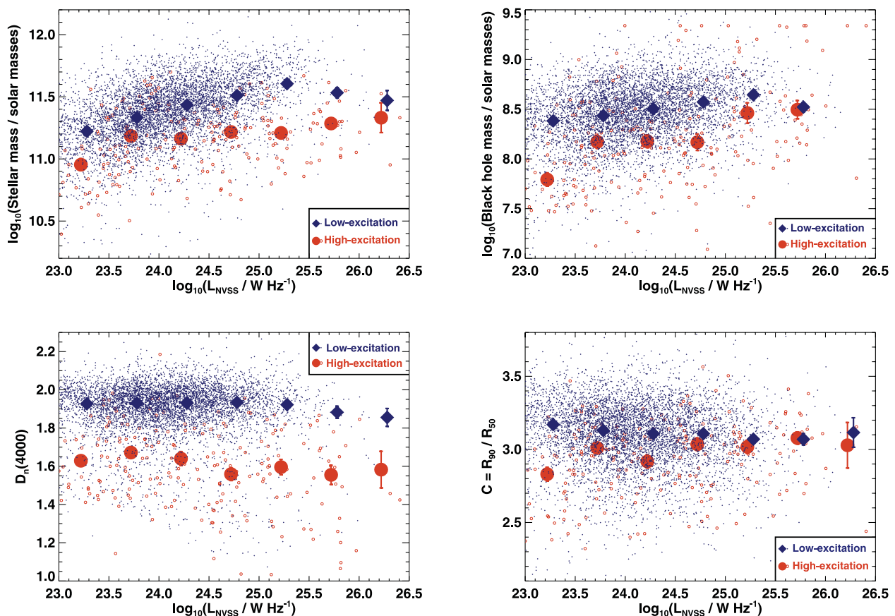
Figure 7. The distributions of stellar mass (upper left), black hole mass (upper right), 4000 Å break strength (lower left) and concentration index ( C = R_{90}/R_{50} , where R_{90} and R_{50} are the radii containing 90 and 50 per cent of the light, respectively; lower right), as a function of radio luminosity, for the LERG and HERG populations separately. The larger symbols indicate the mean values for each population in radio luminosity bins.
