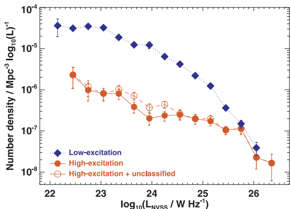
Figure 4. The local radio luminosity function at 1.4 GHz, derived separately for the HERG and LERG populations. Note how both populations are found across the full range of radio luminosities studied.
