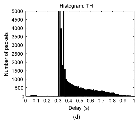
Fig. 6. Histograms of RTT delays measured from ADAC Laboratory at NCSU to: (a) www.lib.ncsu.edu ; (b) www.visitnc.com ; (c) www.utexas.edu ; (d) www.ku.ac.th .
