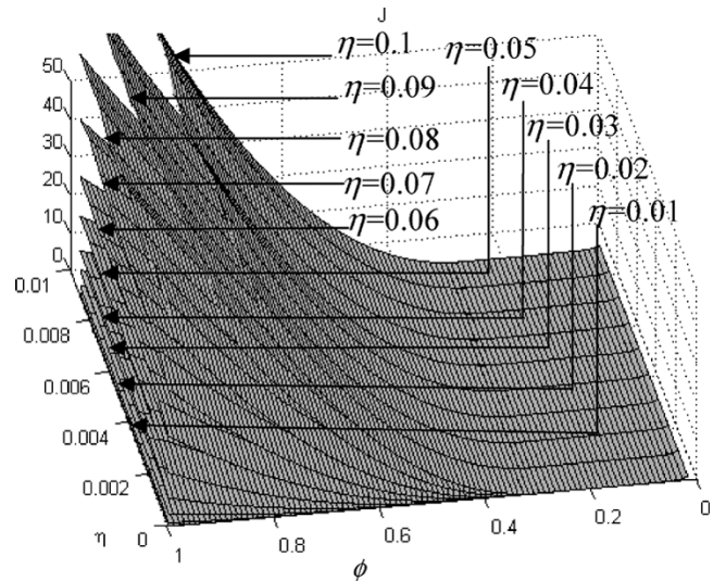
Fig. 8. Typical cost surfaces of J with respect to various \eta and \phi without constraint.
