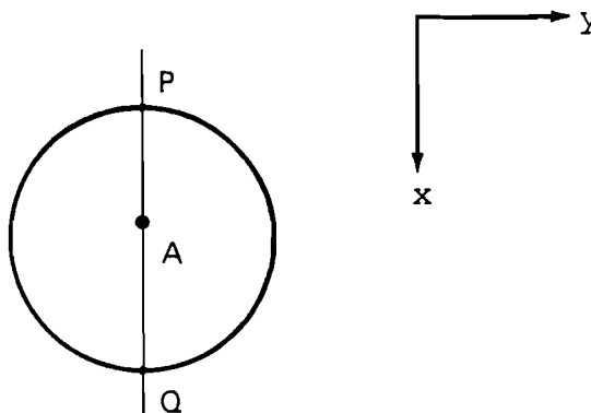
Figure 2.2. An isochrone in the velocity field V(x) = \omega x .
