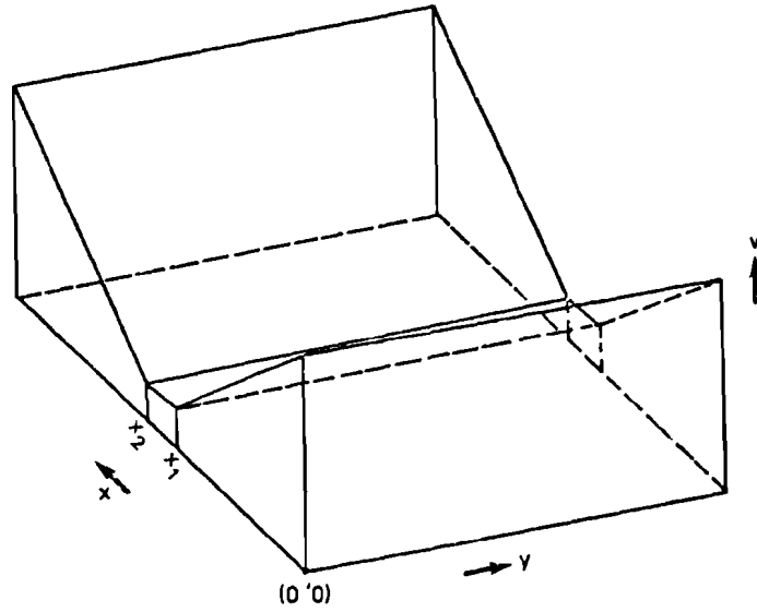
(a) A profile of the velocity field, where the strip between x_1 and x_2 represents the obstruction.
