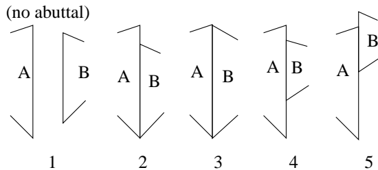
Figure 2: Five possible ways in which two sides of polygonal atoms A and B in a partition can abut. We disregard abutments that occur at only one point.
