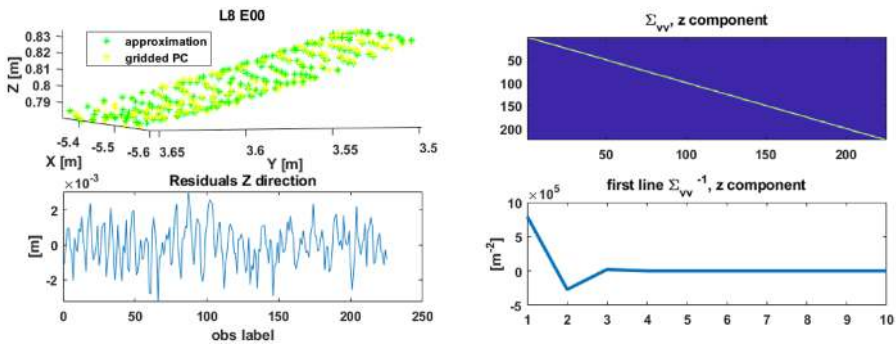
Fig. 4 Top left: the gridded point clouds (yellow) and the approximation (green) for L8. Bottom left: the z-residuals. Top right: scaled Toeplitz VCM \hat{\Sigma}_{\hat{v},z} estimated from the z-component. Bottom right: first ten values of the first row of \hat{\Sigma}_{\hat{v},z}^{-1}
