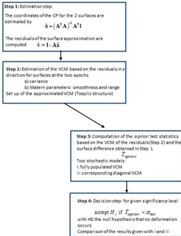
Fig. 1 Methodology of the congruence test using an estimation of the covariance structure from the residuals of the LS approximation
