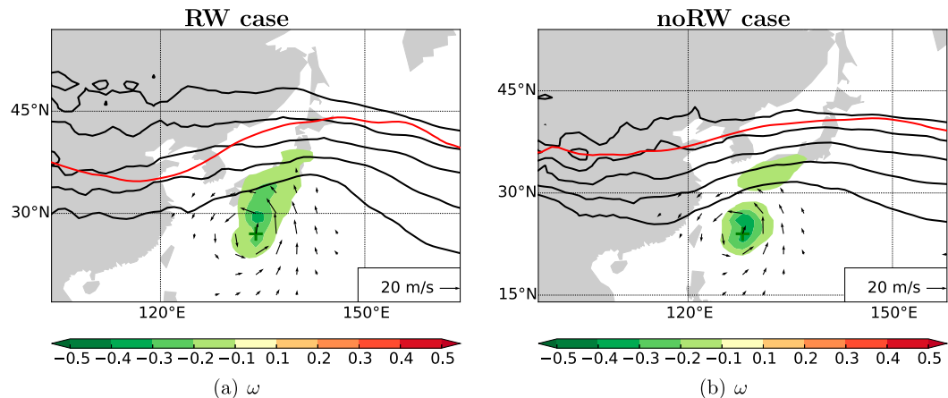
FIG. 11. (a) RW case and (b) no-RW case TC-relative composite analyses of 700–500-hPa vertical velocity (shading in \text{Pa s}^{-1} ), 900-hPa winds (vectors in \text{m s}^{-1} ), 900-hPa temperature (black contours from 284 to 292 K with 2-K contour interval), and 320–360-K PV (contoured in red at 2 PVU) at recurvature time. For illustrative purposes the coastlines are shown relative to the mean TC position (green cross).
