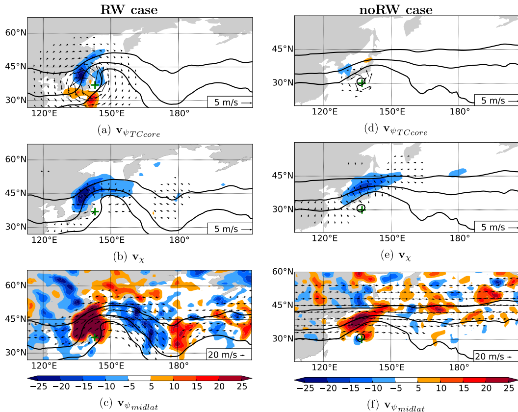
FIG. 14. As in Fig. 10, but 2 days after recurvature.
