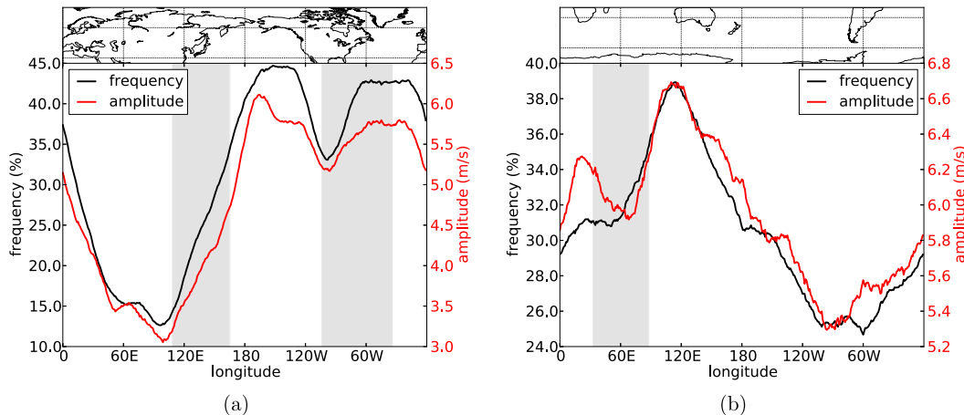
FIG. 2. Mean RWP frequency (%) and mean RWP amplitude ( \text{m s}^{-1} ) (a) over the Northern Hemisphere and (b) over the Southern Hemisphere during June–November and December–April, respectively. Note the different scale for the y axes in (a),(b). The gray shading indicates the range of longitudes of recurring TCs that are included in this study.
