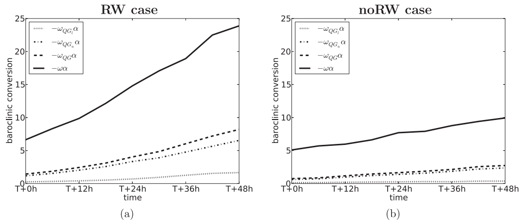
FIG. 13. (a) RW case and (b) no-RW case average baroclinic conversion through low-level forced QG ascent ( -\omega_{QG_l}\alpha ), upper-level forced QG ascent ( -\omega_{QG_u}\alpha ), the full QG ascent ( -\omega_{QG}\alpha ), and the model vertical wind field ( -\omega\alpha ) in \text{W m}^{-2} between recurvature time and 2 days after recurvature. The box over which the average was performed is shown in Figs. 12 and 16.
