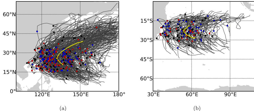
FIG. 1. Best tracks of (a) WNP TCs and (b) south Indian Ocean TCs that fulfill the criteria given in section 2a (source: International Best Track Archive for Climate Stewardship). Circles denote the position of each TC at recurvature time. Circles are colored by decade: 1980–89 (black), 1990–99 (red), and 2000–10 (blue). The yellow line gives the mean recurring track ( T - 48 to T + 96 h) and the yellow star denotes the mean recurvature point.
