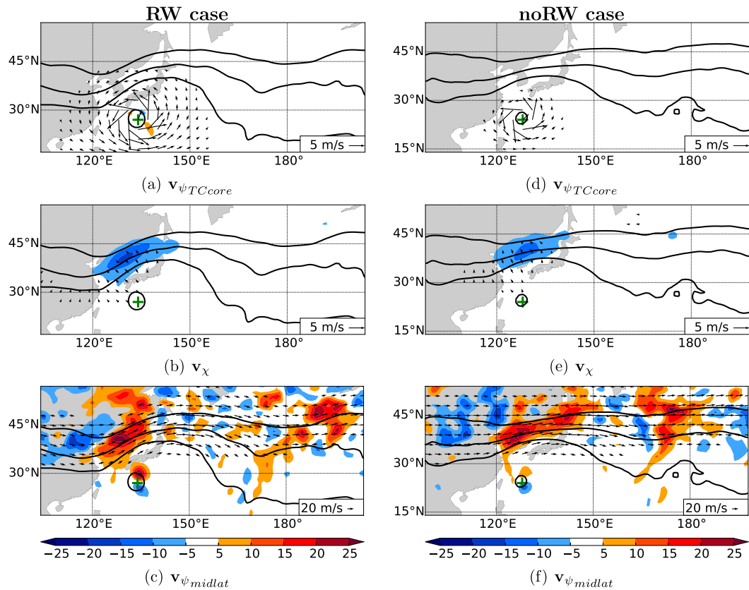
FIG. 10. (a)–(c) RW case and (d)–(f) no-RW case TC-relative composite analyses of 320–360-K PV (contoured in black at 1, 2, and 4 PVU) ( 1 \text{ PVU} = 10^{-6} \text{ K kg}^{-1} \text{ m}^2 \text{ s}^{-1} ) and 320–360-K PV advection (shaded in 10^{-6} PVU s^{-1} ) induced by the 320–360-K winds given at bottom right (vectors in \text{m s}^{-1} ) at recurvature time. For illustrative purposes the coastlines are shown relative to the mean TC position (green cross).
