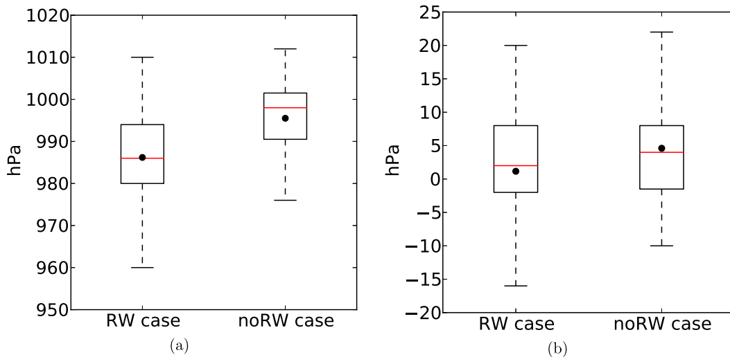
FIG. 19. As in Fig. 9, but for the (a) mean sea level pressure (hPa) at the time when the RW case TCs and no-RW case TCs were first classified as extratropical cyclone and the (b) mean sea level pressure change (hPa) between the time of classification as extratropical cyclone and the end of the best track.
