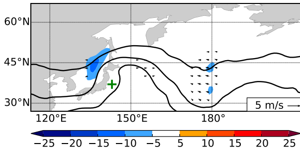
FIG. 17. As in Fig. 14b, but negative PV advection by divergent wind forced through QG vertical motion.
