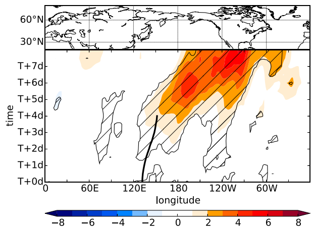
FIG. 21. Recurvature-relative composites of the anomaly of 250-hPa geopotential height ensemble standard deviation (shaded in gpm) relative to June–November climatology for WNP TCs. Values that are statistically significant at the 95% confidence level are hatched. Black thick line gives the mean recurving track ( T + 0 to T + 96 h).
