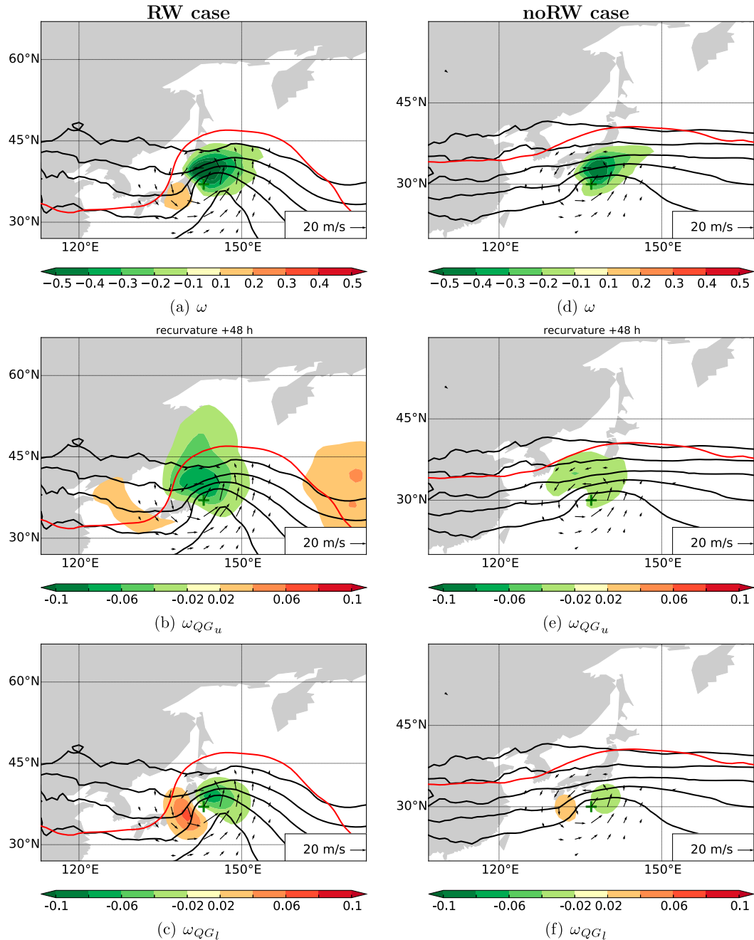
FIG. 15. As in Fig. 11, but showing 700–500-hPa (a),(d) total vertical velocity (shading in \text{Pa s}^{-1} ); (b),(e) QG vertical velocity forced from upper troposphere (500–100 hPa); and (c),(f) QG vertical velocity forced from lower troposphere (1000–750 hPa) 2 days after recurvature. Note the different color bar used for (a) and (d).
