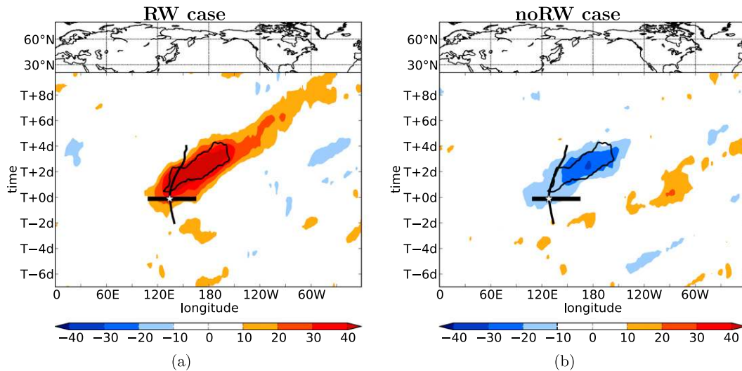
FIG. 6. Anomaly of RWP frequency (shaded in %) relative to June–November climatology for (a) RW case and (b) no-RW case for the WNP TCs. The black contour indicates the mask that we used to determine the lower and upper quintile (56 events). The black thick line gives the mean recurring track ( T - 48 to T + 96 h) for each case and the white star denotes the mean recurvature point. Black horizontal bar marks the range of longitudes of the TCs at recurvature. Data are smoothed with a Gaussian filter.
