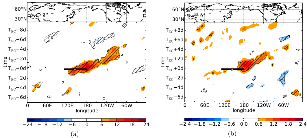
FIG. 4. As in Fig. 3, but relative to the time T_{EC} + 0 day when the TCs were first classified as an extratropical cyclone by the RSMC. Black horizontal bar marks the range of longitudes of the TCs at T_{EC} . White star marks the mean longitude of all TCs at T_{EC} .
