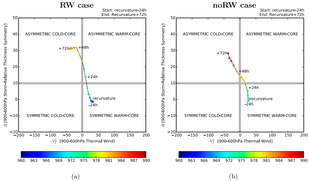
FIG. 20. Cyclone phase space diagram for the (a) RW case TC and (b) the no-RW case TC from 1 day prior to recurvature to 3 days after recurvature. Phase evolution of -V_T^2 versus B . A marker is placed every 6 h. The color of each marker denotes the cyclone mean sea level pressure (hPa) according to the best track data.
