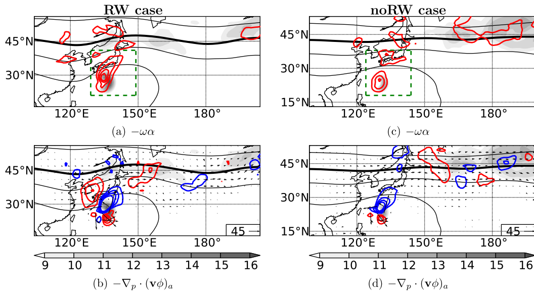
FIG. 12. (a),(b) RW case and (c),(d) no-RW case TC-relative composite analyses of vertically integrated K_e (shaded in 10^5 \text{ J m}^{-2} ), 200 hPa geopotential (contoured in black at 200 \text{ m}^2 \text{ s}^{-2} intervals, thick black line illustrates 11\,800 \text{ m}^2 \text{ s}^{-2} isoline), and vertically integrated K_e budget terms given in subcaptions (colored contours at 8 \text{ W m}^{-2} intervals) at recurvature time. (b),(d) Ageostrophic geopotential flux vectors (reference vector in 10^6 \text{ W m}^{-1} ). The green box in (a),(c) shows the region over which the mean baroclinic conversion was computed. For illustrative purposes the coastlines are shown relative to the mean TC position.
