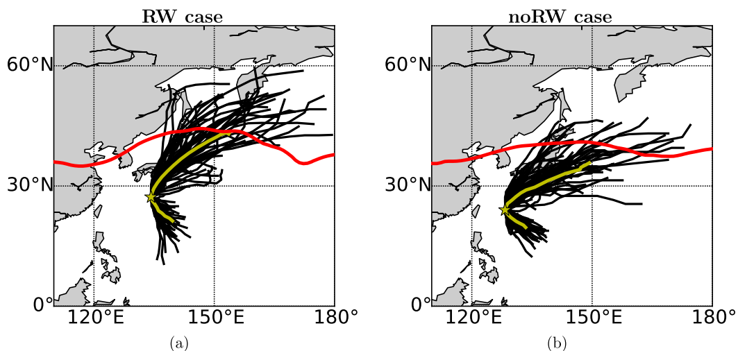
FIG. 18. 320–360-K PV (contoured in red at 2 PVU) and best tracks of (a) the RW case TCs and (b) the no-RW case TCs in a recurvature-relative framework. The yellow line gives the mean recurring track ( T - 48 to T + 96 h) and the yellow star denotes the mean recurvature point. For illustrative purposes the coastlines are shown relative to the mean TC position at recurvature time.
