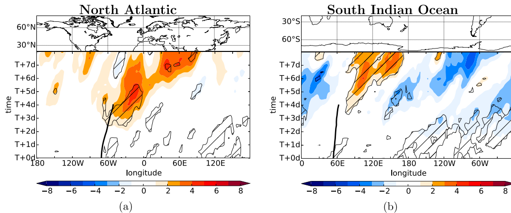
FIG. 23. As in Fig. 21, but for (a) North Atlantic and (b) south Indian Ocean TCs relative to June–November and December–April climatology, respectively.
