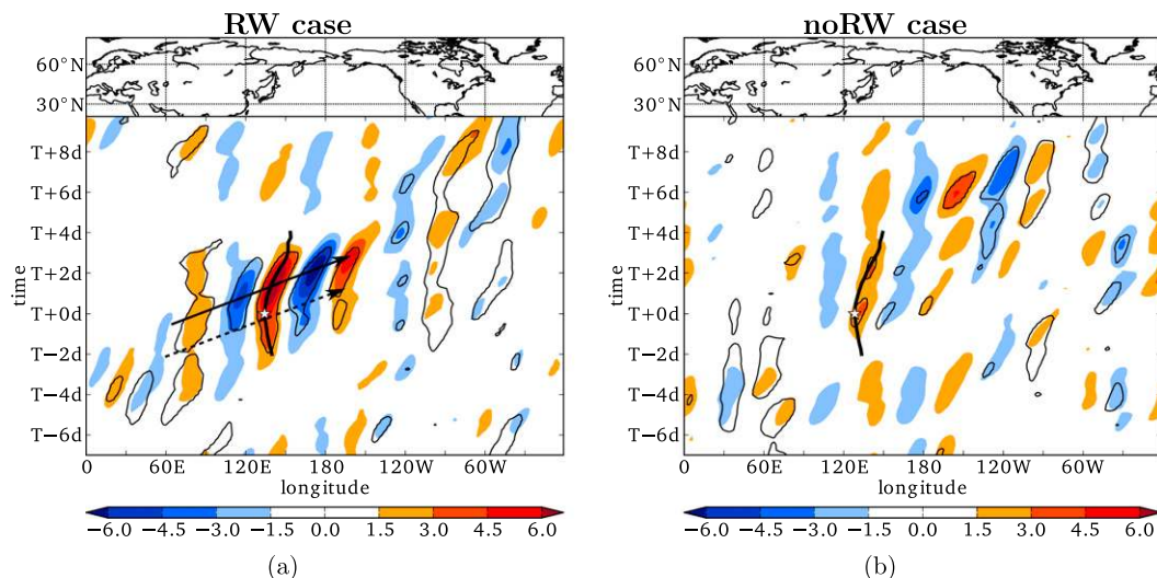
FIG. 7. (a) RW case and (b) no-RW case recurvature-relative composite Hovmöller diagrams of the 20^\circ – 80^\circ\text{N} -averaged 250-hPa meridional wind (shaded in \text{m s}^{-1} ) for zonal wavenumbers 5–15. Black contours denote the statistical significance at the 99% confidence level based on a two-sided Student's t test. The black thick line gives the mean recurring track ( T - 48 to T + 96 h) for each case and the white star denotes the mean recurvature point. The dashed and solid black arrows in (a) indicate the estimated zonal group velocity of the Rossby wave based on the leading edge and the peak amplitude, respectively.
