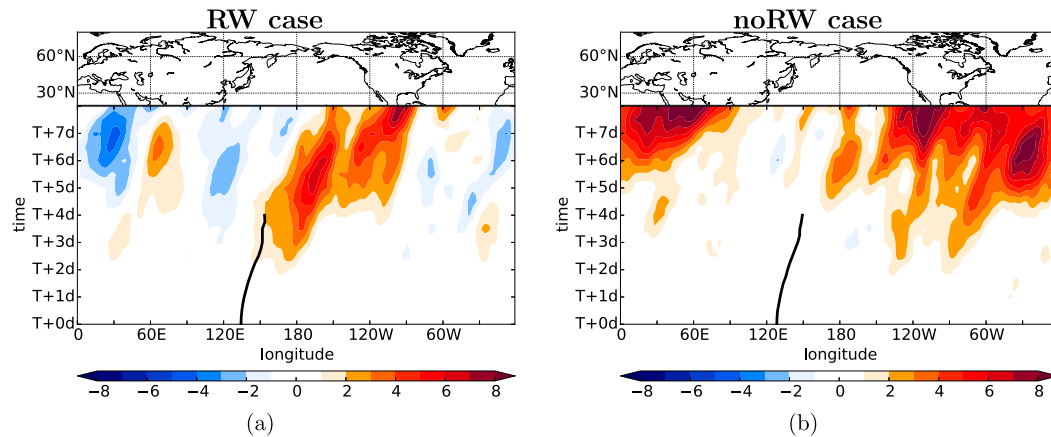
FIG. 22. Recurvature-relative composites of the anomaly of 250-hPa geopotential height ensemble standard deviation (shaded in gpm) relative to June–November climatology for WNP (a) RW case and (b) no-RW case TCs. Black thick line gives the mean recurring track ( T + 0 to T + 96 h).
