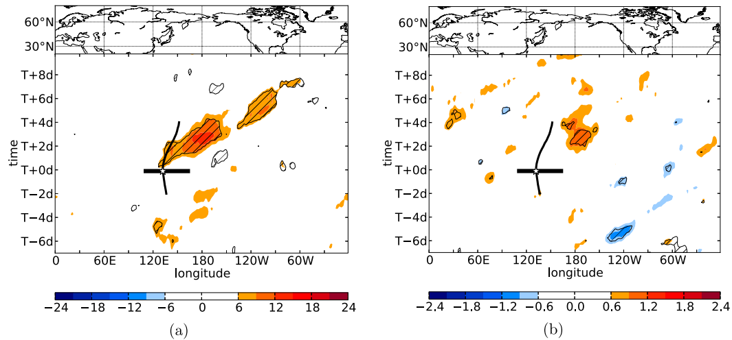
FIG. 3. Recurvature-relative composites of (a) RWP frequency anomaly (shaded in %) and (b) RWP amplitude anomaly (shaded in \text{m s}^{-1} ) relative to June–November climatology for WNP TCs. Values that are statistically significant at the 95% confidence level are hatched. Black thick line gives the mean recurving track ( T - 48 to T + 96 h) and the white star denotes the mean recurvature point. Black horizontal bar marks the range of longitudes of the TCs at recurvature. Data are smoothed with a Gaussian filter.
