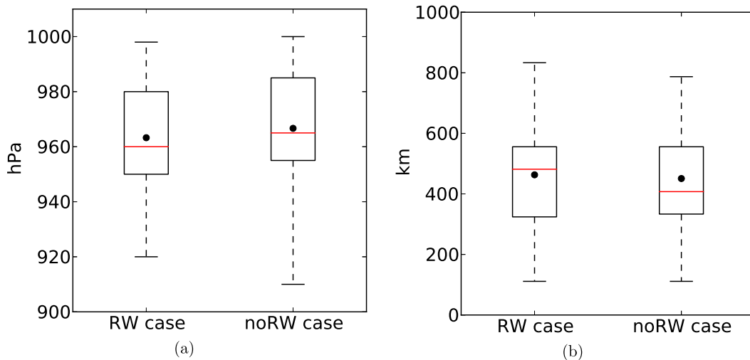
FIG. 9. Box plots showing (a) mean sea level pressure (hPa) and (b) length of the maximum 15.4 \text{ m s}^{-1} wind radius (km) for the RW case TCs and no-RW case TCs at recurvature time. The length of the maximum 15.4 \text{ m s}^{-1} (30 kt) wind radius was derived from the Japan Meteorological Agency best track dataset. The lower and upper bounds of each box give the 25th and 75th percentiles, respectively; the red bar and the black circle inside each box denote the median and mean, respectively; and the whiskers extend from the 25th and 75th percentiles to the 5th and 95th percentiles, respectively.
