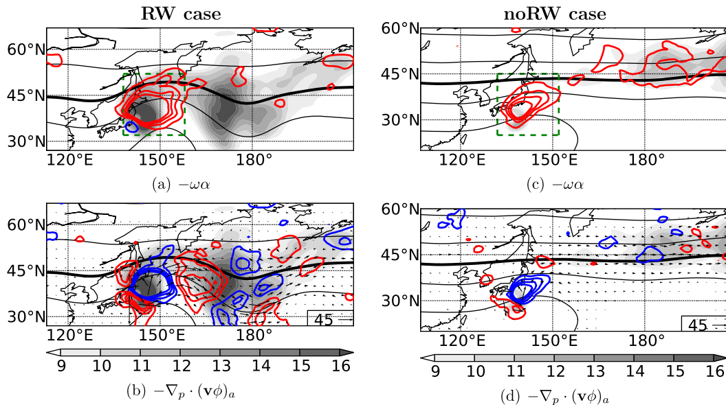
FIG. 16. As in Fig. 12, but 2 days after recurvature.
