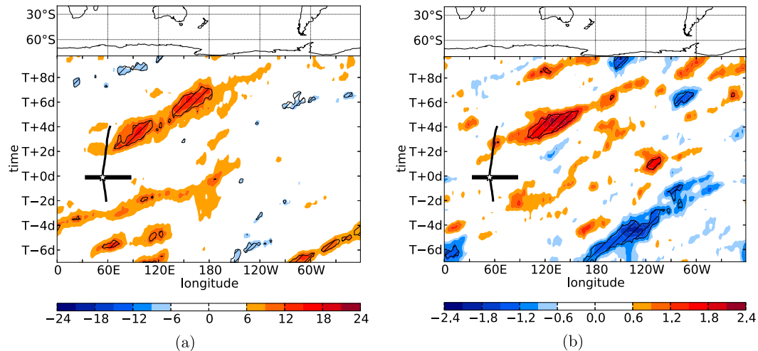
FIG. 5. As in Fig. 3, but for anomaly relative to December–April climatology for the western south Indian Ocean TCs.
