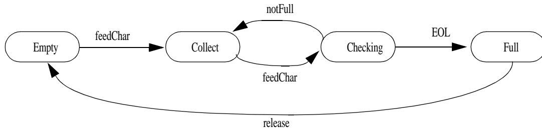
FIGURE 3. The changed WrapAText FSM
