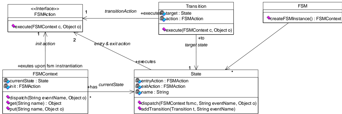
FIGURE 5. Class diagram for the FSM Framework
