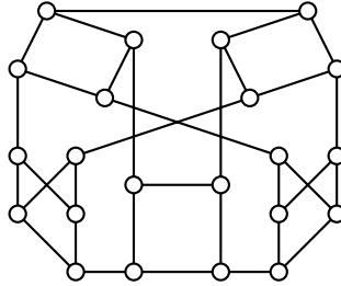
Figure 3: A bipartite cubic graph G with i(G) = 4n/11 .
