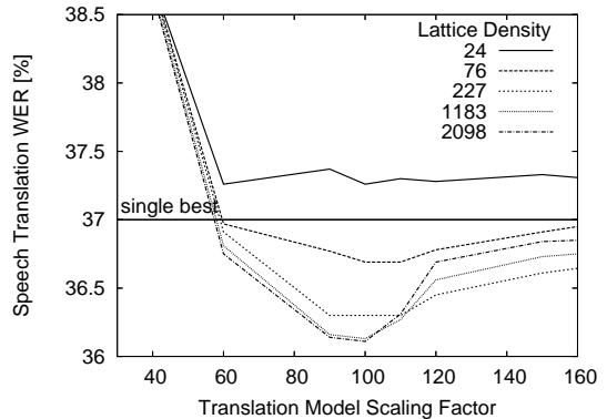
Figure 2: Effect of different lattice densities and translation model scaling factors \lambda on the translation WER (FUB task). Lattices with density 24 were generated using tight beams which resulted in a slightly worse recognition WER.
