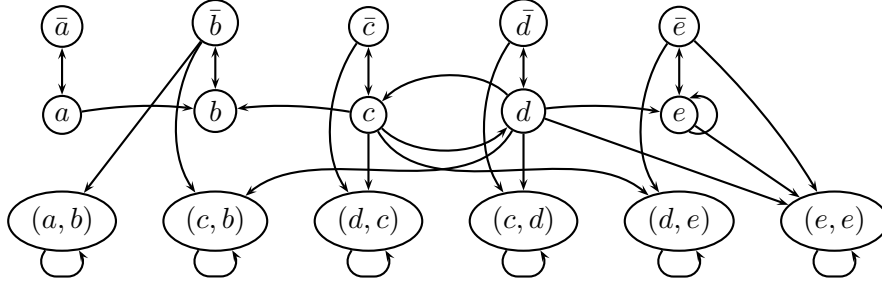
Figure 9: Tr_6(F) for the AF F from Example 1.
