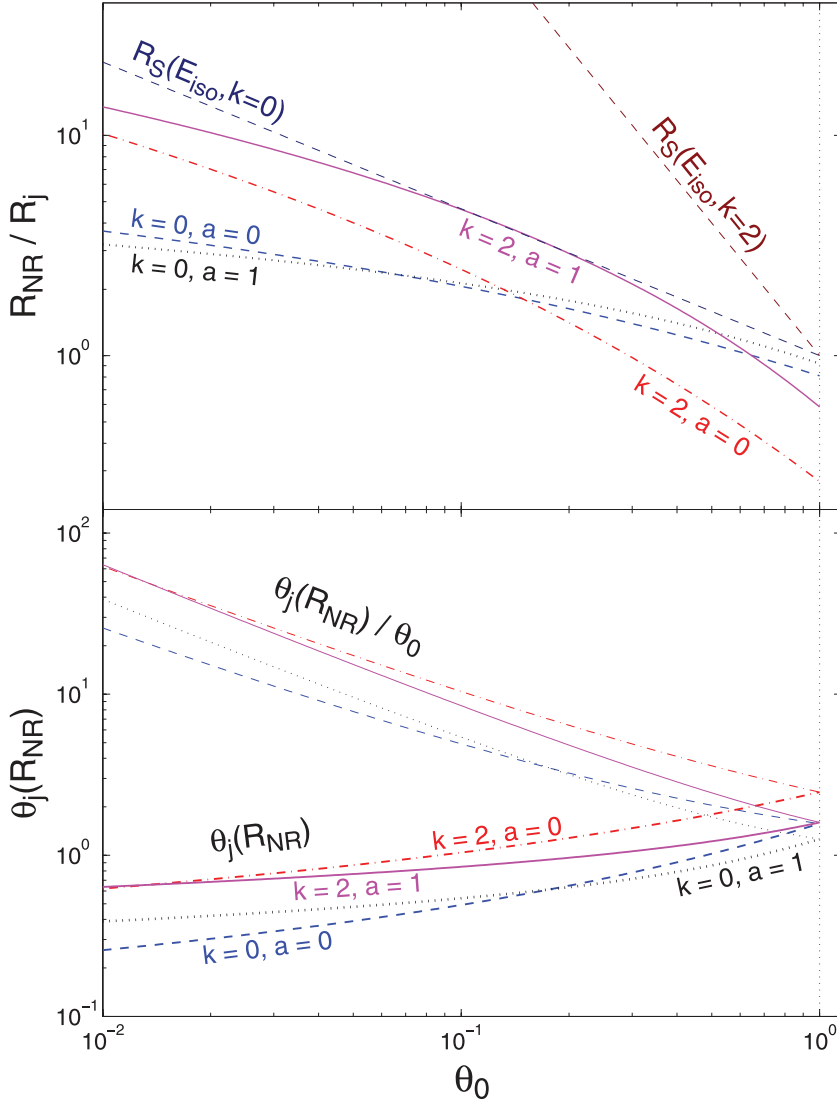
Figure 5. Upper panel: the non-relativistic transition radius for our analytic relativistic model, R_{\text{NR}} , defined by \Gamma(R_{\text{NR}}) = 1 , normalized by R_j , as a function of \theta_0 . For comparison, R_S(E_{\text{iso}}) is also shown; the two radii, R_{\text{NR}} and R_S(E_{\text{iso}}) , become similar at \theta_0 \sim 1 but are very different for \theta_0 \ll 1 . Lower panel: the value of the jet half-opening angle, \theta_j , at R_{\text{NR}} , where our simple analytic relativistic model breaks down.
