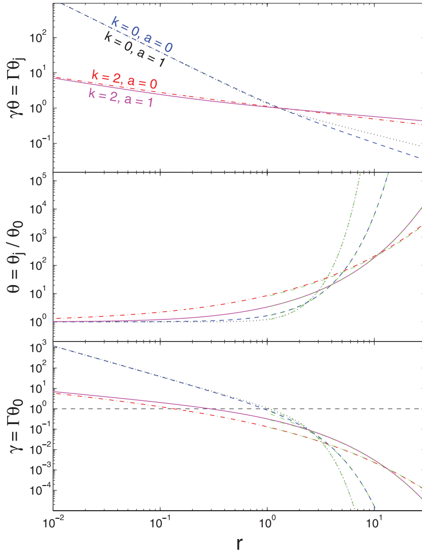
Figure 2. The jet dynamics according to our relativistic analytic model (see text in Section 4 for details), for either a uniform ( k = 0 ) or a wind-like, stratified ( k = 2 ) external density profile, and for either the old ( a = 0 ) or our new ( a = 1 ) recipe for the jet lateral expansion speed. The dynamical range in this figure is unrealistically large, and it is shown mainly in order to demonstrate the properties of this solution, and show how well our analytic approximation for r > 1 works (the dashed green lines in the middle and bottom panels, which are practically on top of the numerical results).
