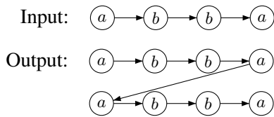
Figure 3: Doubling abba
