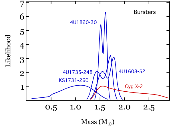
Figure 6. Likelihoods P_i(\text{data}|M_{\text{NS}}) for the accreting bursting neutron stars discussed as category V in the text. The likelihood for Cyg X-2 was inferred using optical observations of its companion star.
