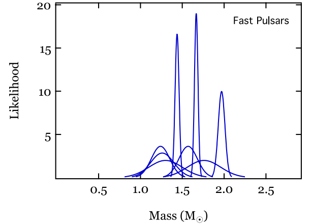
Figure 2. Likelihoods P_i(\text{data}|M_{\text{psr}}) for nine recycled pulsars with white dwarf companions. The measurement of \geq 2 PK parameters in these binaries lead to precisely determined neutron star masses. These systems belong to category Ib discussed in the text.
