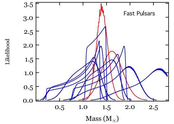
Figure 4. Likelihoods P_i(\text{data}|M) for the recycled neutron stars with one PK parameter (blue curves; category IIb) or with optical observations of the white dwarf companions (red curves; category III).
