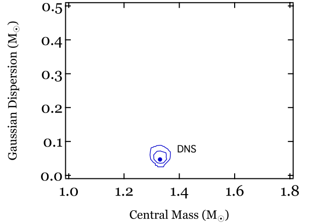
Figure 7. Confidence contours over the parameters of a Gaussian distribution for the double neutron stars.
