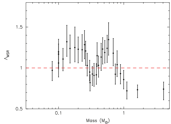
Figure 4. The evolution of the mass segregation ratio, \Lambda_{MSR} , as a function of mass for subsets of 40 stars. We plot the highest mass object in each subset. The dashed line indicates \Lambda_{MSR} = 1 , i.e. no mass segregation.
