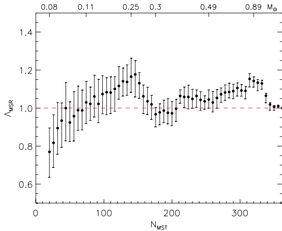
Figure 3. The evolution of the mass segregation ratio, \Lambda_{MSR} , with respect to the N_{MST} least massive stars (brown dwarfs) in Taurus. Error bars show the 1/6th and 5/6th percentile values from the median as described in the text. The dashed line indicates \Lambda_{MSR} = 1 , i.e. no mass segregation. We show the highest mass within N_{MST} stars on the top axis.
